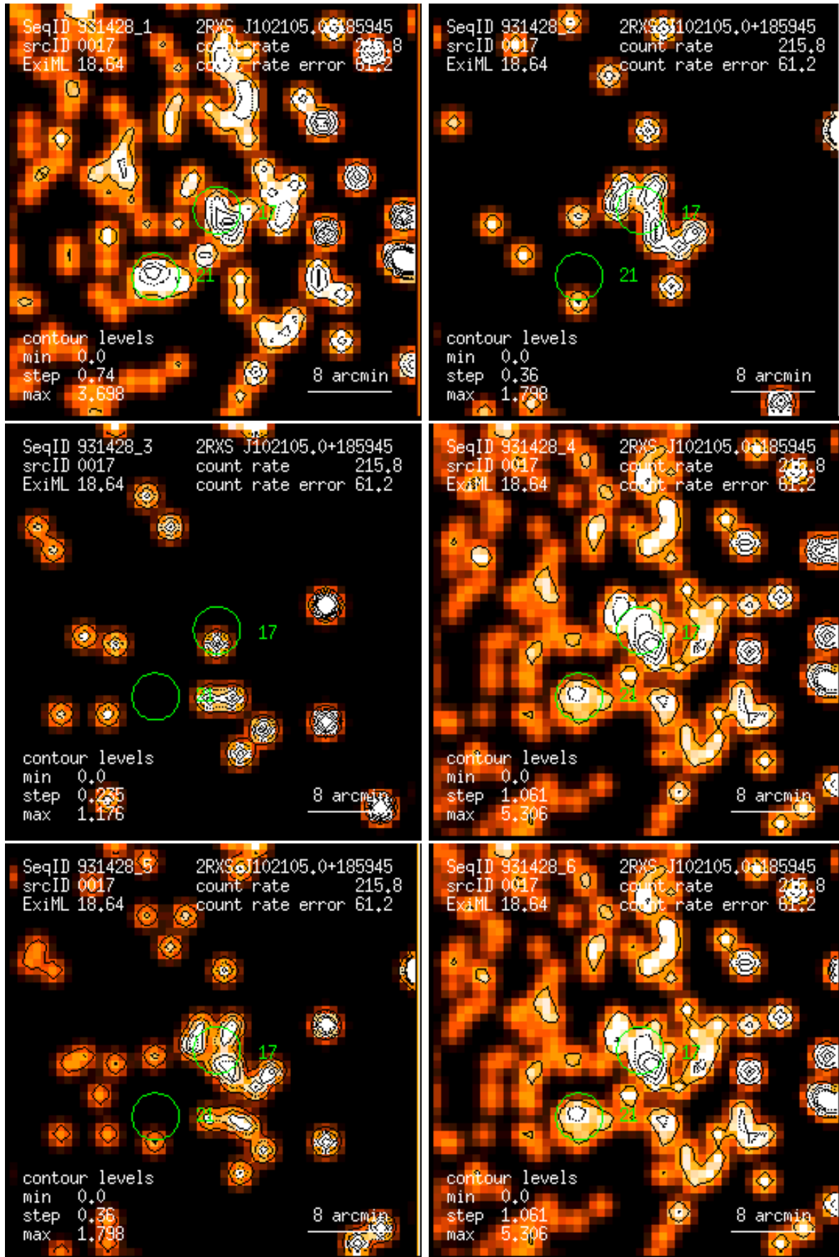
Figure 17: RASS 931428: detection 0017: band rate images, Gaussian filter: (1) PSPC channels 11 – 41, (2) 52 – 90, (3) 91 – 201, (4) 11 – 235, (5) 52 – 201, (6) 11 – 201. Broad band rates in counts/ks. Band rate contour levels in counts/ks/arcmin 2 .
