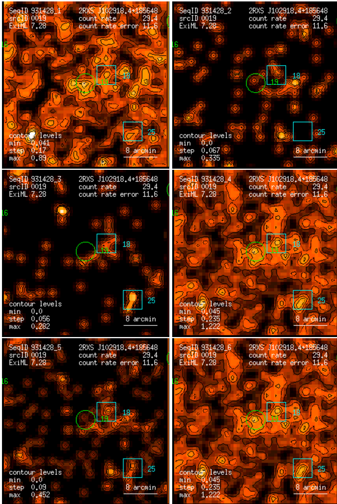
Figure 19: RASS 931428: detection 0019: band rate images, Gaussian filter: (1) PSPC channels 11 – 41, (2) 52 – 90, (3) 91 – 201, (4) 11 – 235, (5) 52 – 201, (6) 11 – 201. Broad band rates in counts/ks. Band rate contour levels in counts/ks/arcmin 2 .
