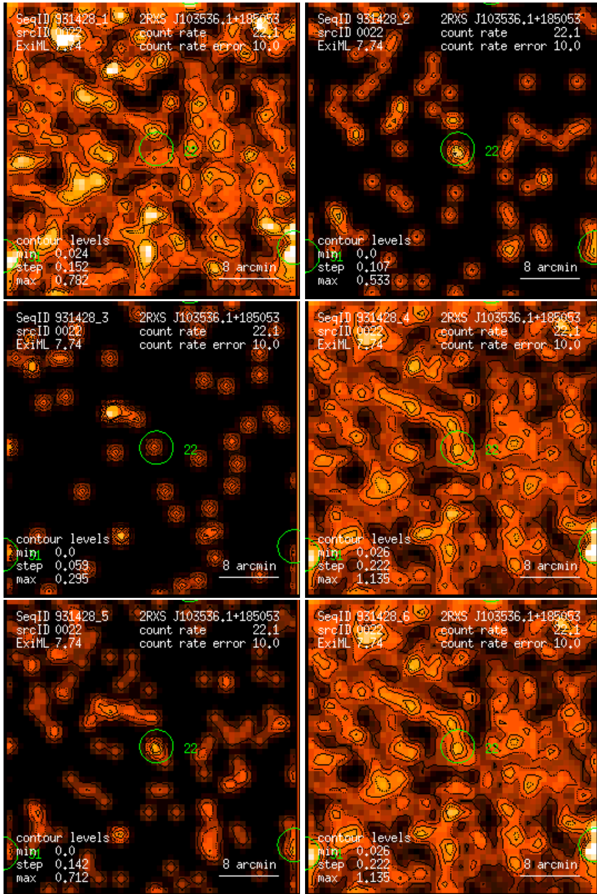
Figure 22: RASS 931428: detection 0022: band rate images, Gaussian filter: (1) PSPC channels 11 – 41, (2) 52 – 90, (3) 91 – 201, (4) 11 – 235, (5) 52 – 201, (6) 11 – 201. Broad band rates in counts/ks. Band rate contour levels in counts/ks/arcmin 2 .
