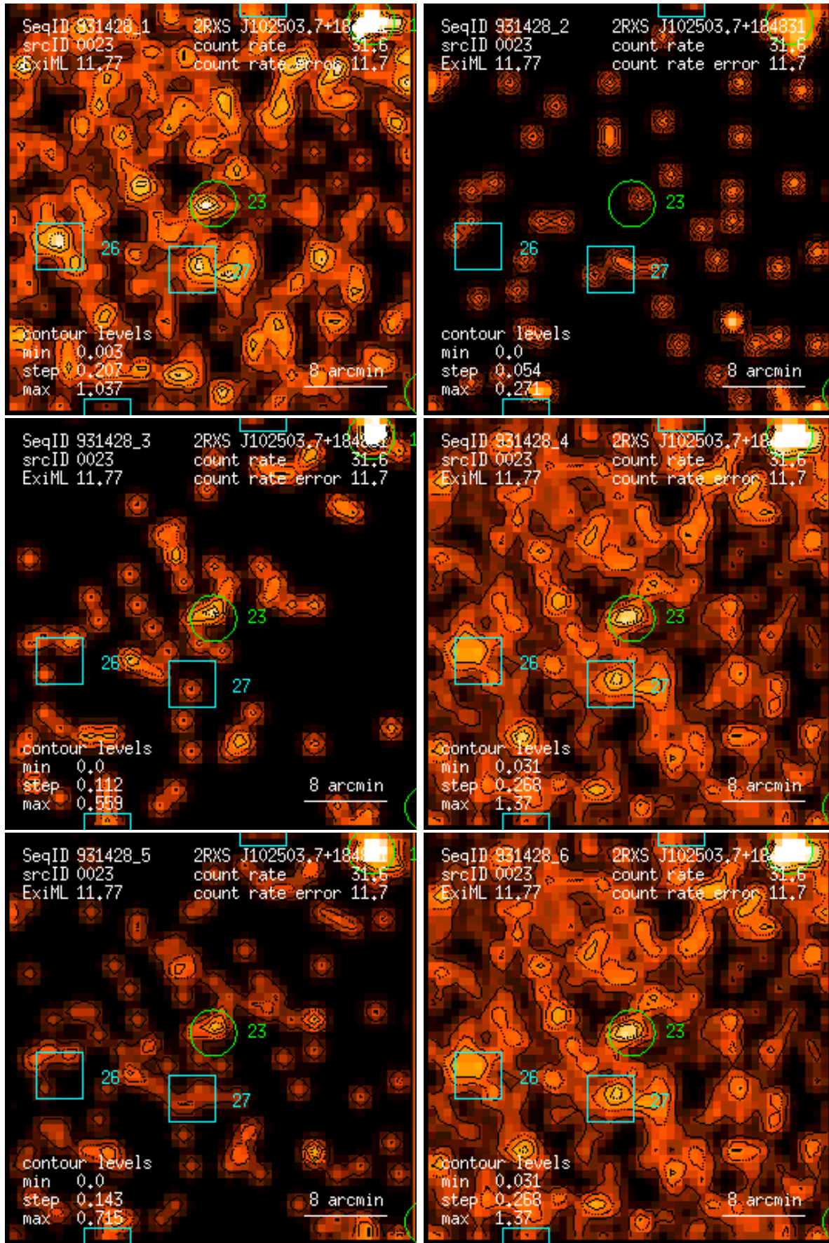
Figure 23: RASS 931428: detection 0023: band rate images, Gaussian filter: (1) PSPC channels 11 – 41, (2) 52 – 90, (3) 91 – 201, (4) 11 – 235, (5) 52 – 201, (6) 11 – 201. Broad band rates in counts/ks. Band rate contour levels in counts/ks/arcmin 2 .
