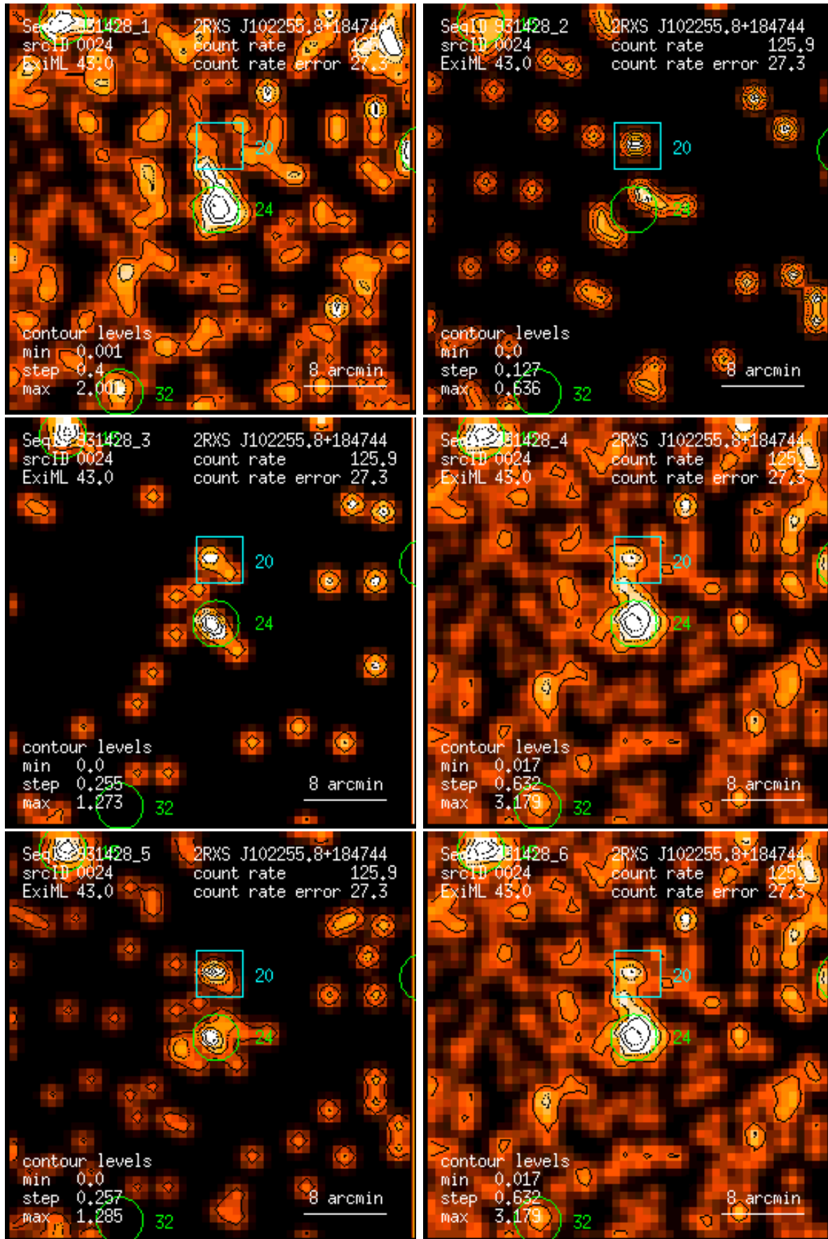
Figure 24: RASS 931428: detection 0024: band rate images, Gaussian filter: (1) PSPC channels 11 – 41, (2) 52 – 90, (3) 91 – 201, (4) 11 – 235, (5) 52 – 201, (6) 11 – 201. Broad band rates in counts/ks. Band rate contour levels in counts/ks/arcmin 2 .
