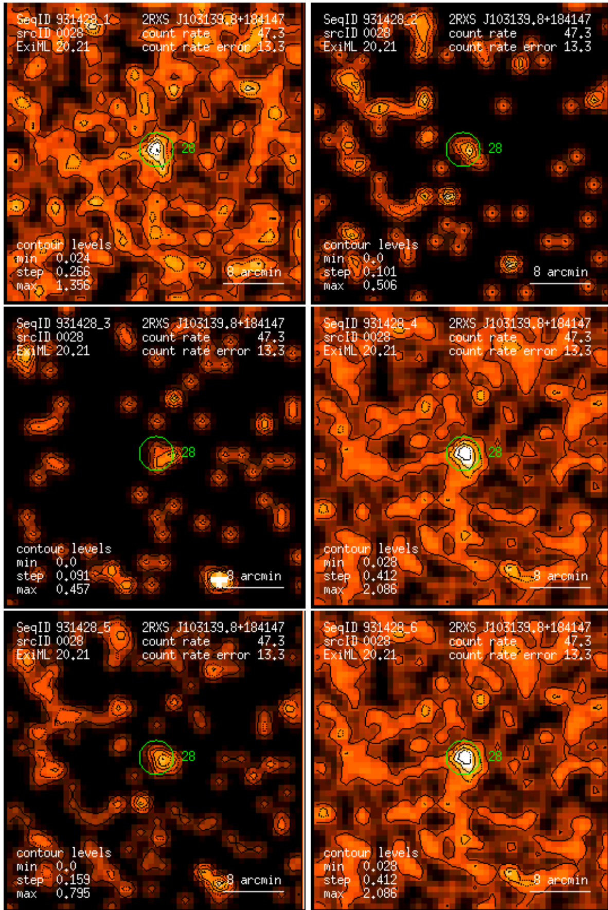
Figure 28: RASS 931428: detection 0028: band rate images, Gaussian filter: (1) PSPC channels 11 – 41, (2) 52 – 90, (3) 91 – 201, (4) 11 – 235, (5) 52 – 201, (6) 11 – 201. Broad band rates in counts/ks. Band rate contour levels in counts/ks/arcmin 2 .
