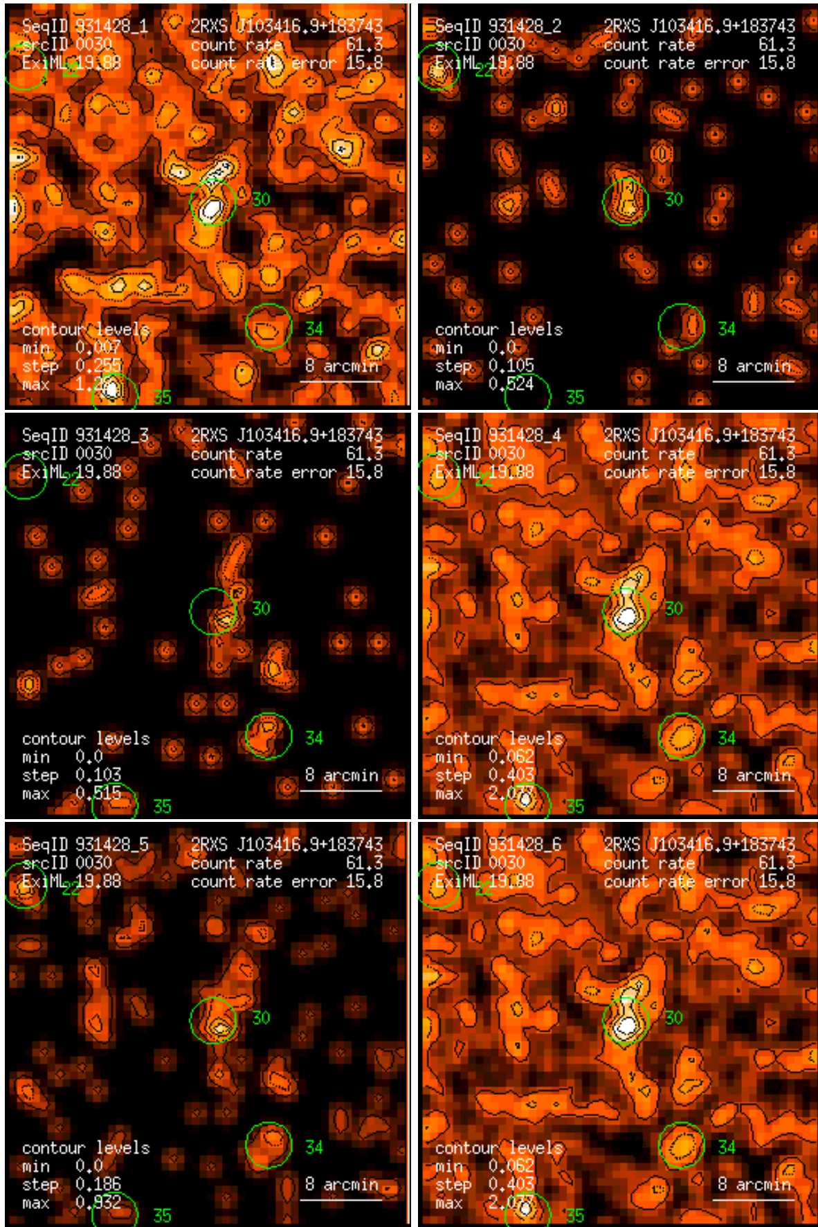
Figure 30: RASS 931428: detection 0030: band rate images, Gaussian filter: (1) PSPC channels 11 – 41, (2) 52 – 90, (3) 91 – 201, (4) 11 – 235, (5) 52 – 201, (6) 11 – 201. Broad band rates in counts/ks. Band rate contour levels in counts/ks/arcmin 2 .
