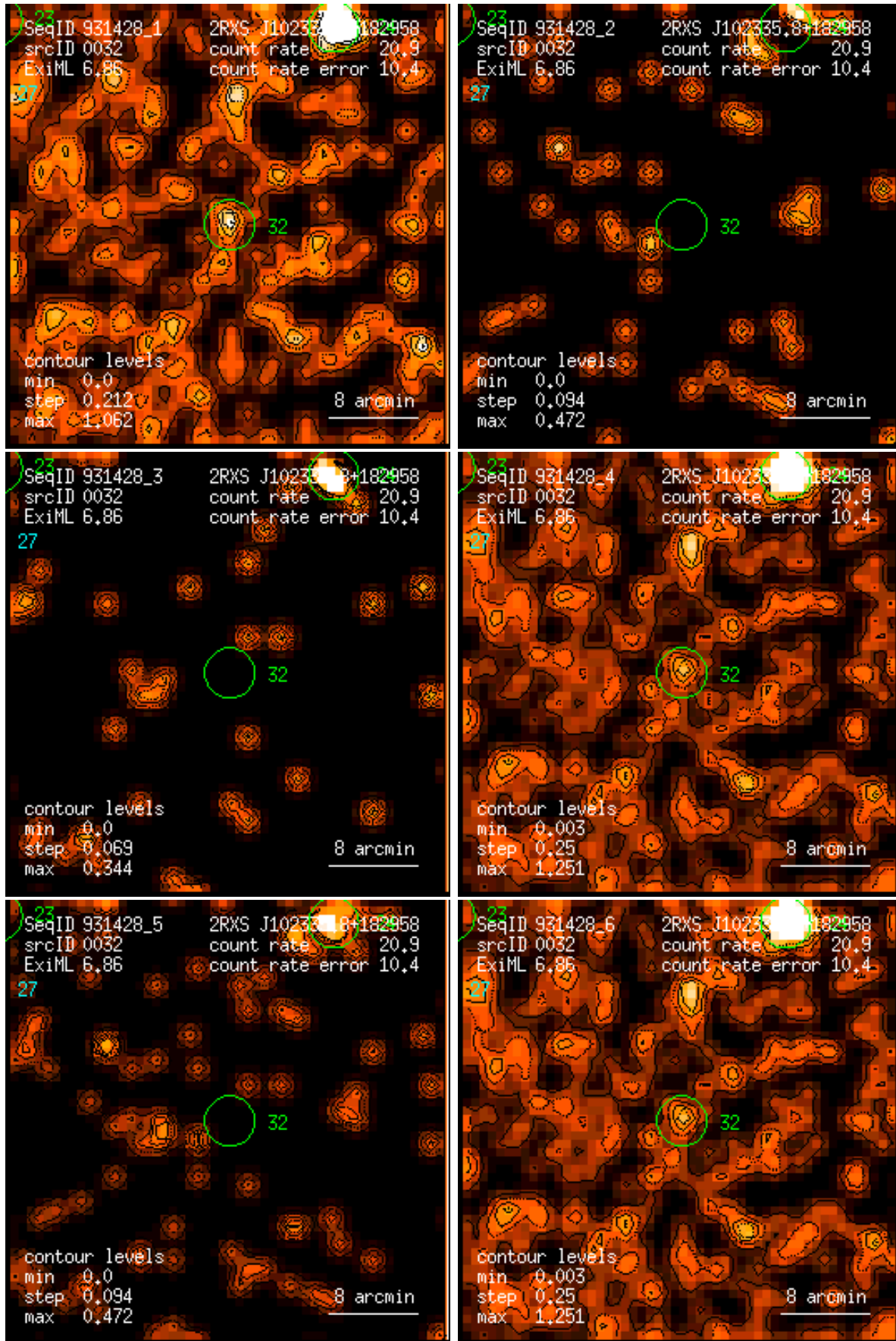
Figure 32: RASS 931428: detection 0032: band rate images, Gaussian filter: (1) PSPC channels 11 – 41, (2) 52 – 90, (3) 91 – 201, (4) 11 – 235, (5) 52 – 201, (6) 11 – 201. Broad band rates in counts/ks. Band rate contour levels in counts/ks/arcmin 2 .
