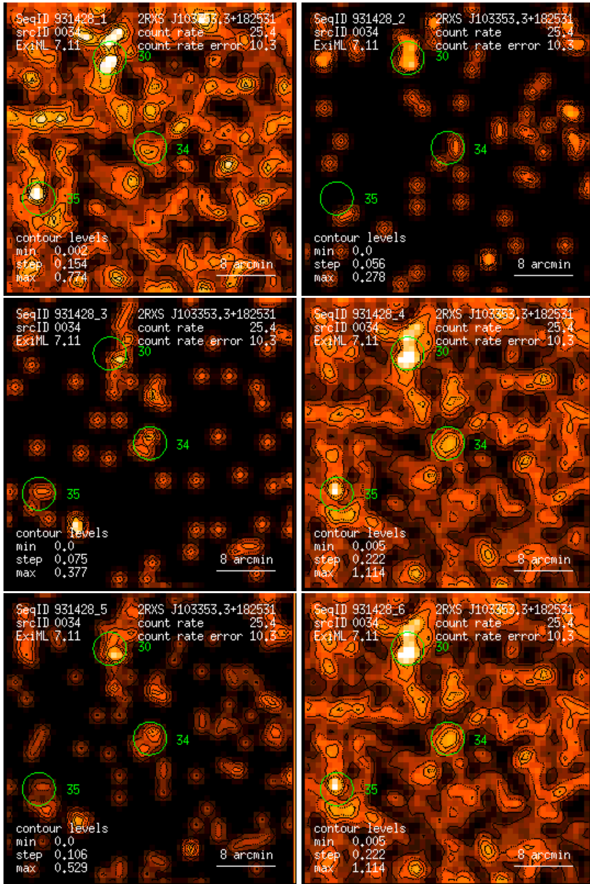
Figure 34: RASS 931428: detection 0034: band rate images, Gaussian filter: (1) PSPC channels 11 – 41, (2) 52 – 90, (3) 91 – 201, (4) 11 – 235, (5) 52 – 201, (6) 11 – 201. Broad band rates in counts/ks. Band rate contour levels in counts/ks/arcmin 2 .
