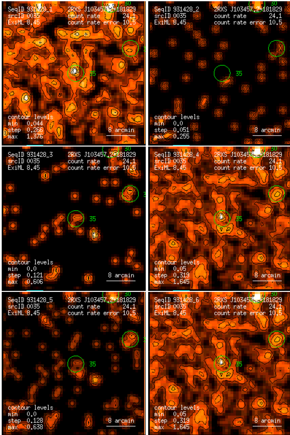
Figure 35: RASS 931428: detection 0035: band rate images, Gaussian filter: (1) PSPC channels 11 – 41, (2) 52 – 90, (3) 91 – 201, (4) 11 – 235, (5) 52 – 201, (6) 11 – 201. Broad band rates in counts/ks. Band rate contour levels in counts/ks/arcmin 2 .
