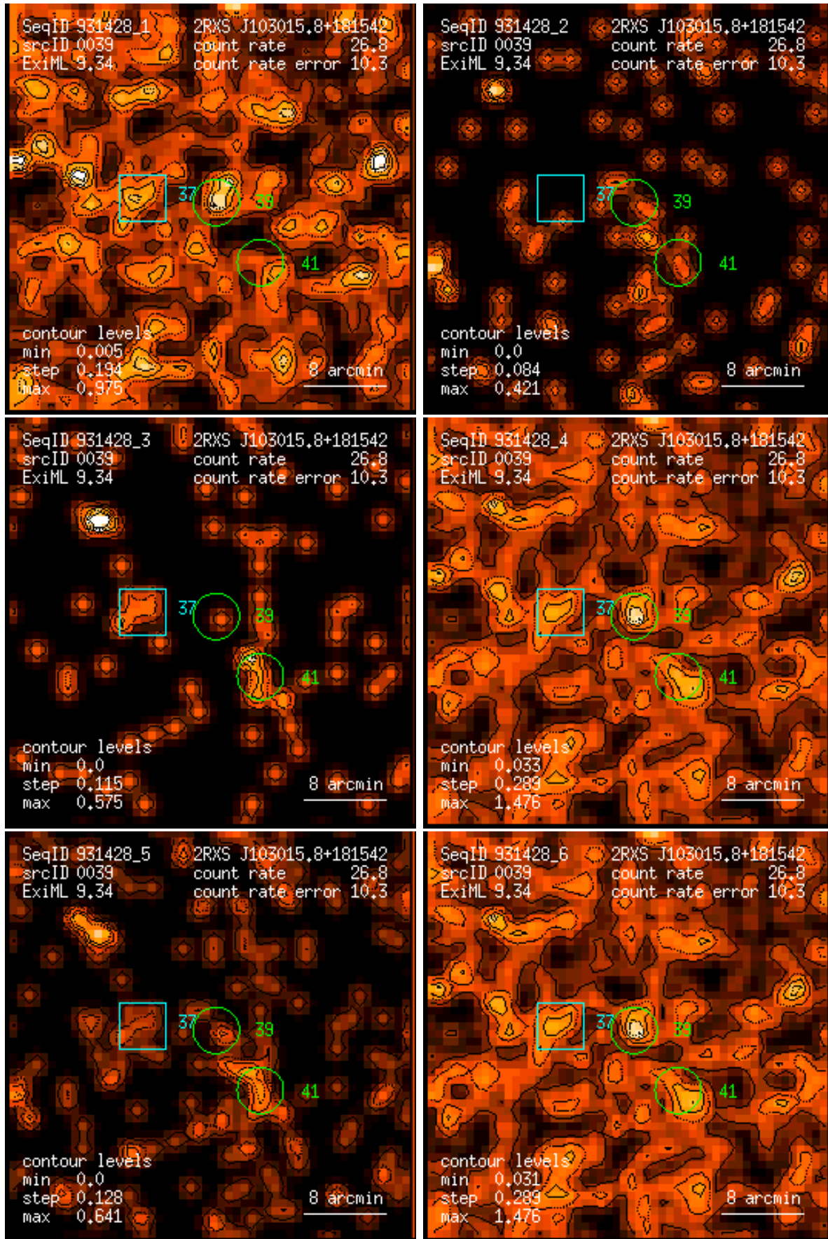
Figure 39: RASS 931428: detection 0039: band rate images, Gaussian filter: (1) PSPC channels 11 – 41, (2) 52 – 90, (3) 91 – 201, (4) 11 – 235, (5) 52 – 201, (6) 11 – 201. Broad band rates in counts/ks. Band rate contour levels in counts/ks/arcmin 2 .
