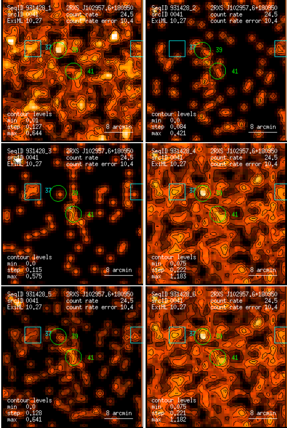
Figure 41: RASS 931428: detection 0041: band rate images, Gaussian filter: (1) PSPC channels 11 – 41, (2) 52 – 90, (3) 91 – 201, (4) 11 – 235, (5) 52 – 201, (6) 11 – 201. Broad band rates in counts/ks. Band rate contour levels in counts/ks/arcmin 2 .
