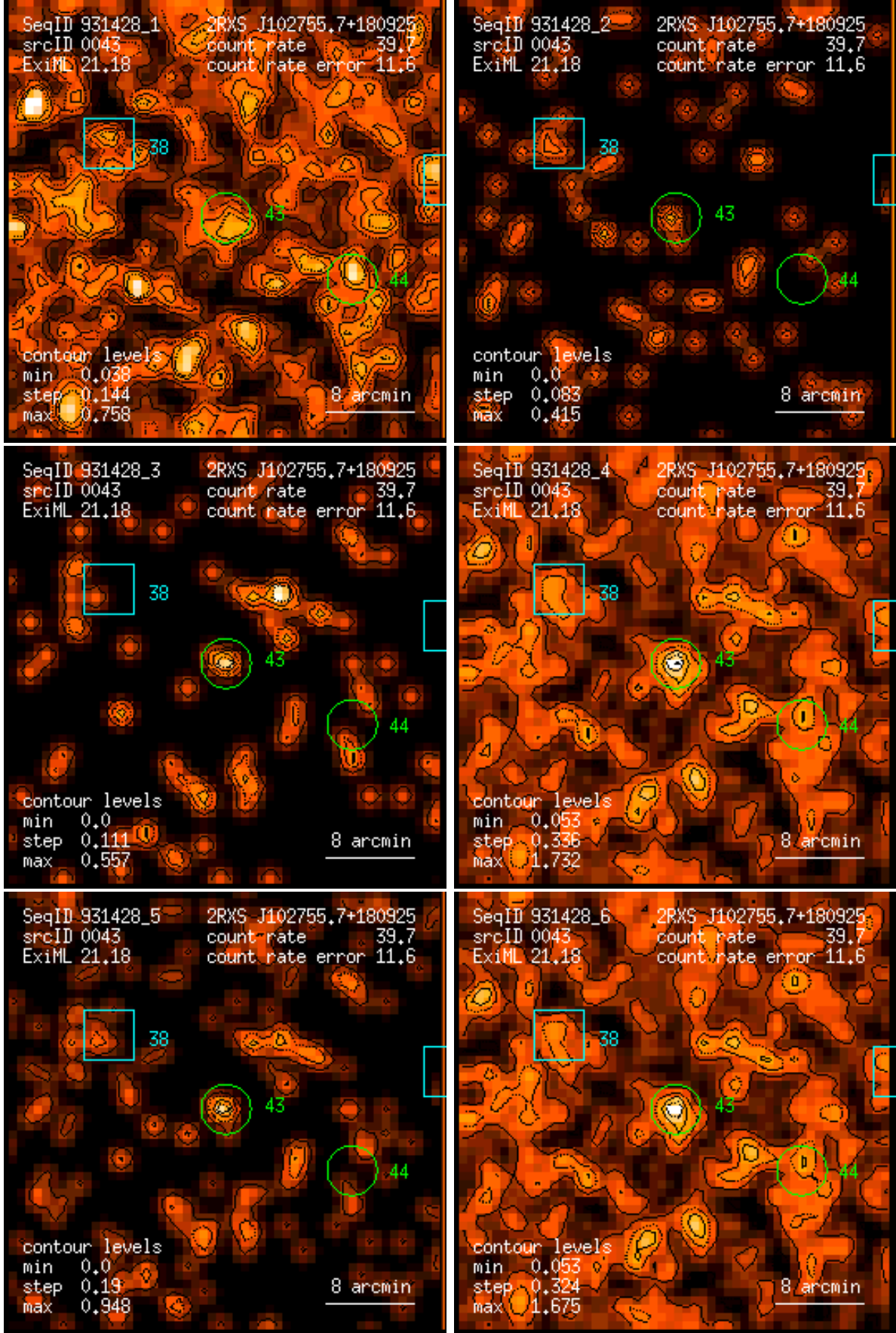
Figure 43: RASS 931428: detection 0043: band rate images, Gaussian filter: (1) PSPC channels 11 – 41, (2) 52 – 90, (3) 91 – 201, (4) 11 – 235, (5) 52 – 201, (6) 11 – 201. Broad band rates in counts/ks. Band rate contour levels in counts/ks/arcmin 2 .
