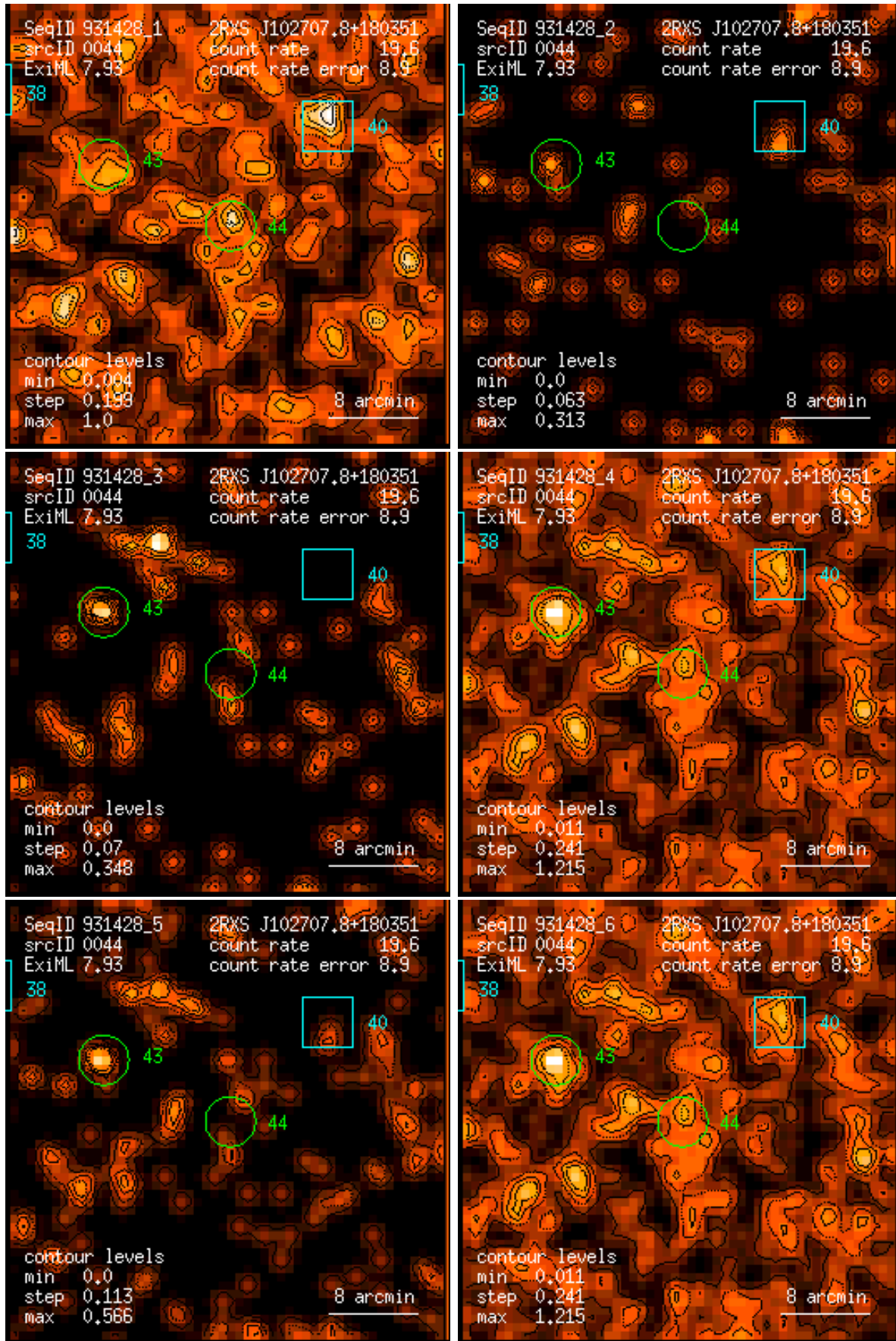
Figure 44: RASS 931428: detection 0044: band rate images, Gaussian filter: (1) PSPC channels 11 – 41, (2) 52 – 90, (3) 91 – 201, (4) 11 – 235, (5) 52 – 201, (6) 11 – 201. Broad band rates in counts/ks. Band rate contour levels in counts/ks/arcmin 2 .
