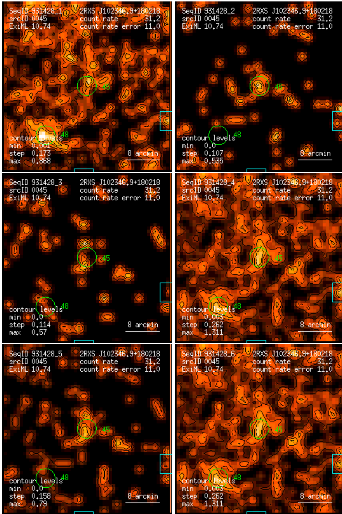
Figure 45: RASS 931428: detection 0045: band rate images, Gaussian filter: (1) PSPC channels 11 – 41, (2) 52 – 90, (3) 91 – 201, (4) 11 – 235, (5) 52 – 201, (6) 11 – 201. Broad band rates in counts/ks. Band rate contour levels in counts/ks/arcmin 2 .
