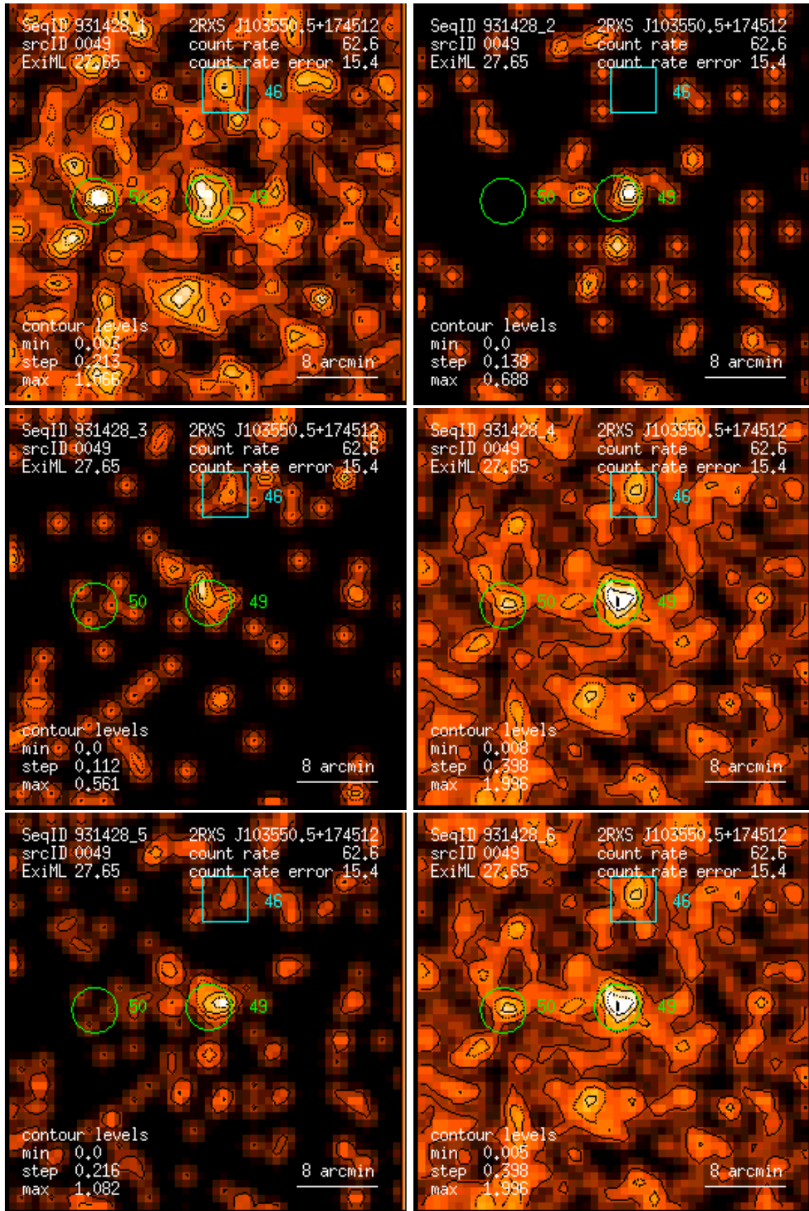
Figure 49: RASS 931428: detection 0049: band rate images, Gaussian filter: (1) PSPC channels 11 – 41, (2) 52 – 90, (3) 91 – 201, (4) 11 – 235, (5) 52 – 201, (6) 11 – 201. Broad band rates in counts/ks. Band rate contour levels in counts/ks/arcmin 2 .
