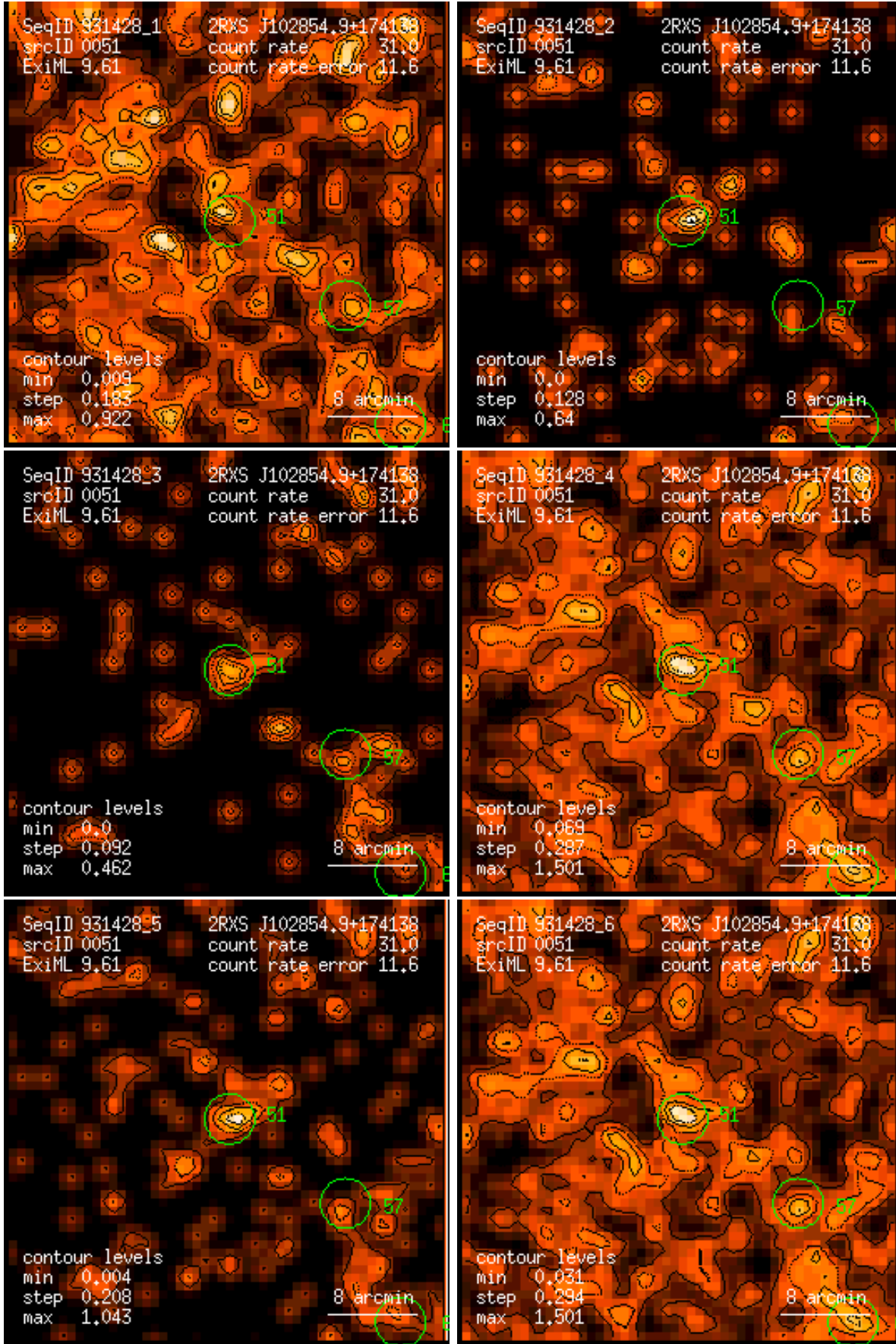
Figure 51: RASS 931428: detection 0051: band rate images, Gaussian filter: (1) PSPP channels 11 – 41, (2) 52 – 90, (3) 91 – 201, (4) 11 – 235, (5) 52 – 201, (6) 11 – 201. Broad band rates in counts/ks. Band rate contour levels in counts/ks/arcmin 2 .
