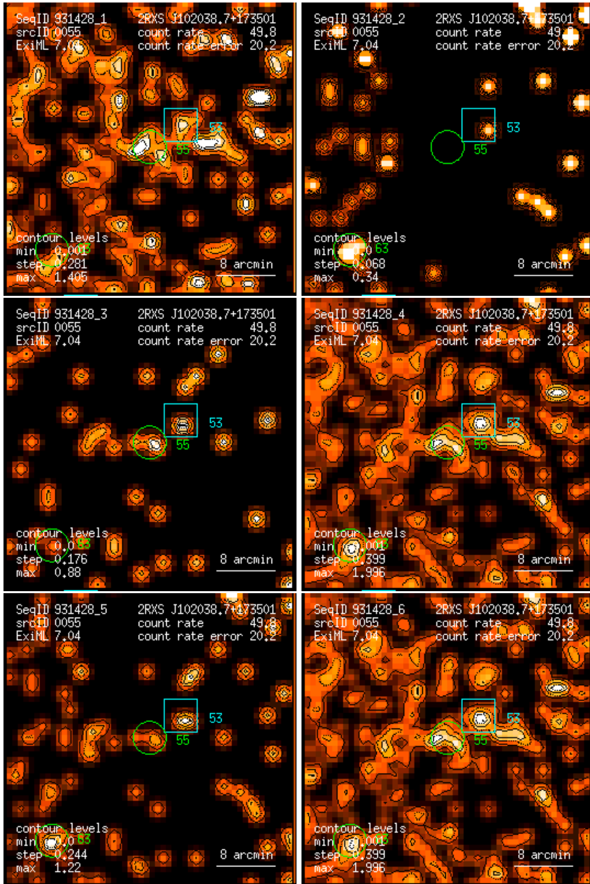
Figure 55: RASS 931428: detection 0055: band rate images, Gaussian filter: (1) PSPC channels 11 – 41, (2) 52 – 90, (3) 91 – 201, (4) 11 – 235, (5) 52 – 201, (6) 11 – 201. Broad band rates in counts/ks. Band rate contour levels in counts/ks/arcmin 2 .
