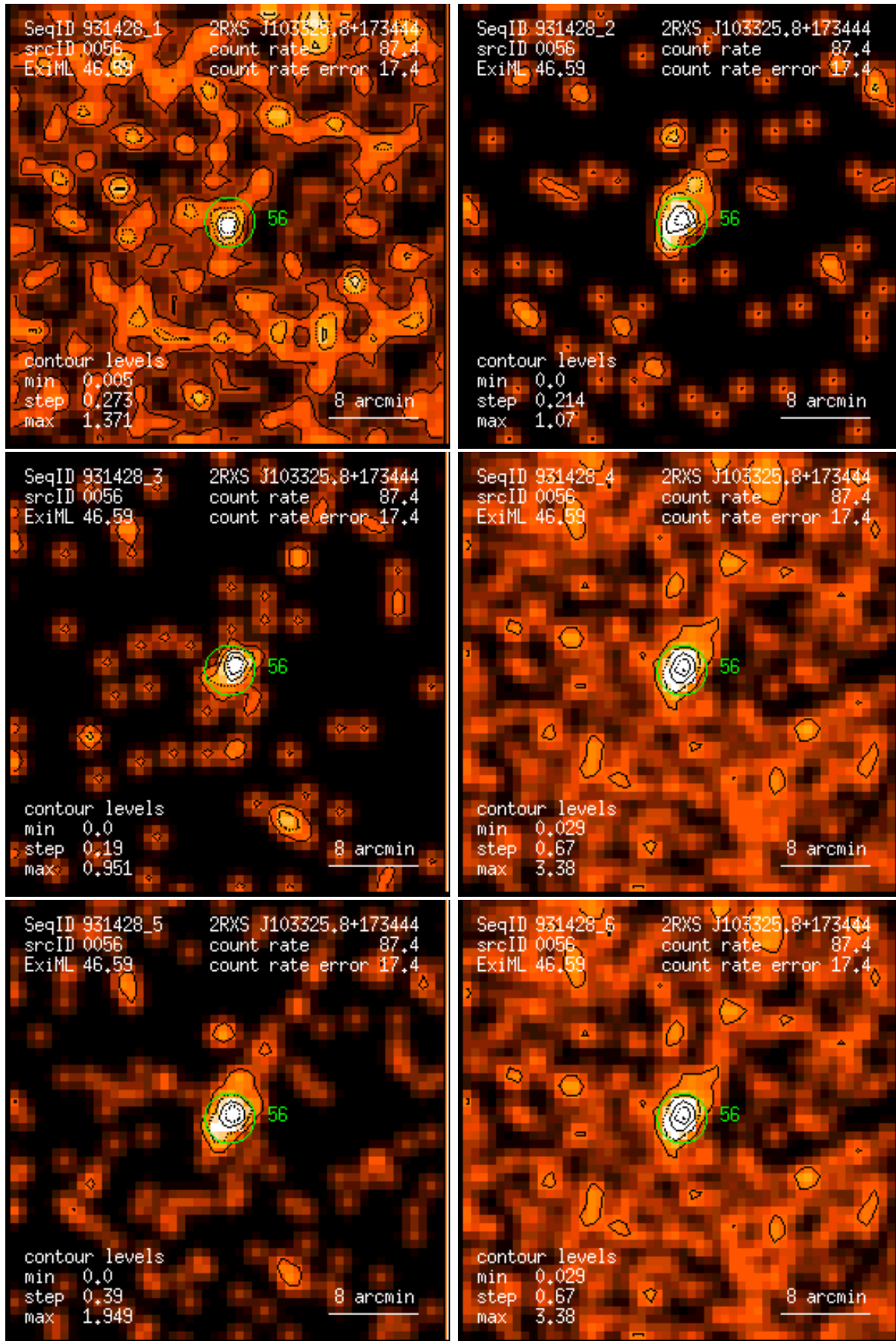
Figure 56: RASS 931428: detection 0056: band rate images, Gaussian filter: (1) PSPC channels 11 – 41, (2) 52 – 90, (3) 91 – 201, (4) 11 – 235, (5) 52 – 201, (6) 11 – 201. Broad band rates in counts/ks. Band rate contour levels in counts/ks/arcmin 2 .
