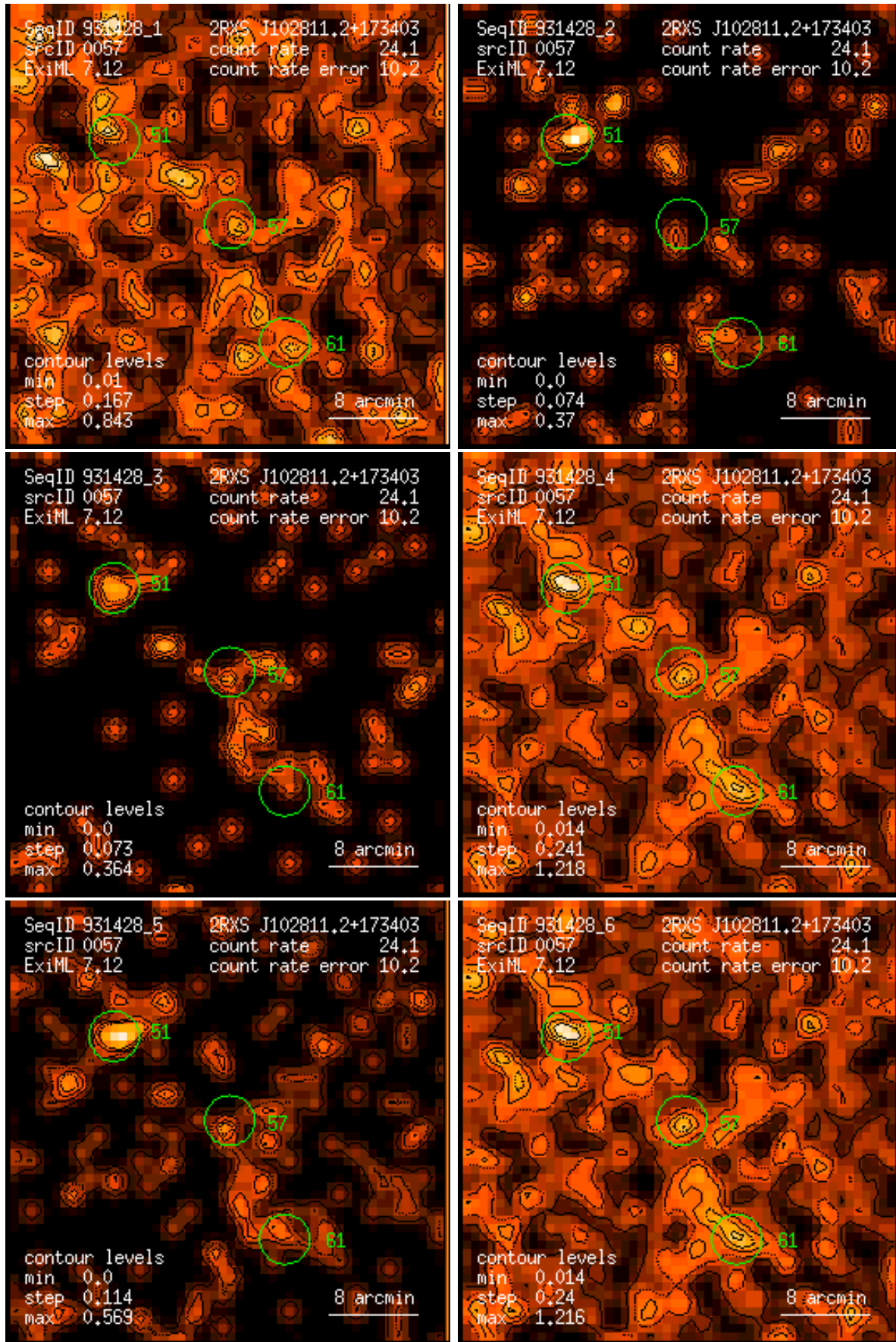
Figure 57: RASS 931428: detection 0057: band rate images, Gaussian filter: (1) PSPC channels 11 – 41, (2) 52 – 90, (3) 91 – 201, (4) 11 – 235, (5) 52 – 201, (6) 11 – 201. Broad band rates in counts/ks. Band rate contour levels in counts/ks/arcmin 2 .
