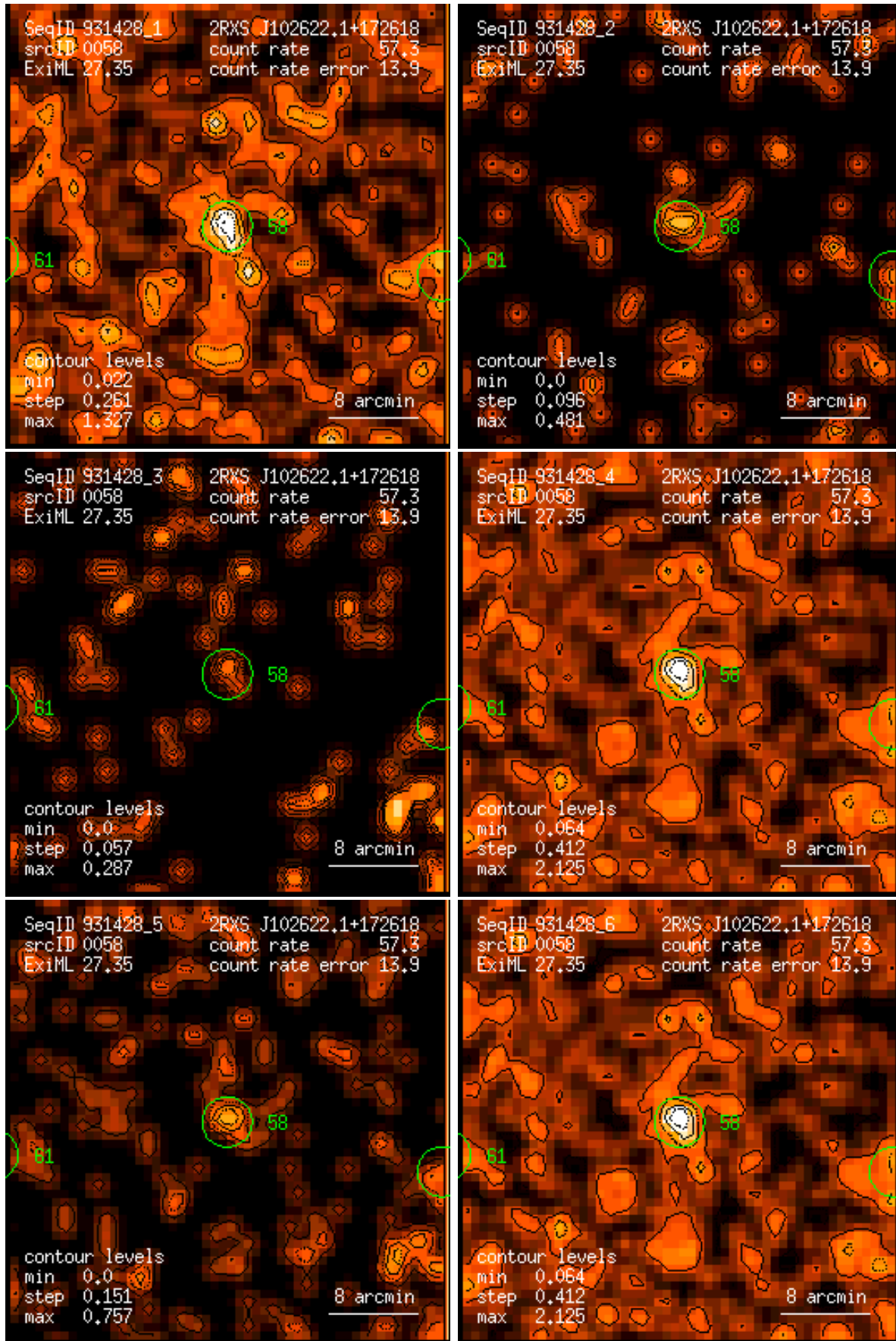
Figure 58: RASS 931428: detection 0058: band rate images, Gaussian filter: (1) PSPC channels 11 – 41, (2) 52 – 90, (3) 91 – 201, (4) 11 – 235, (5) 52 – 201, (6) 11 – 201. Broad band rates in counts/ks. Band rate contour levels in counts/ks/arcmin 2 .
