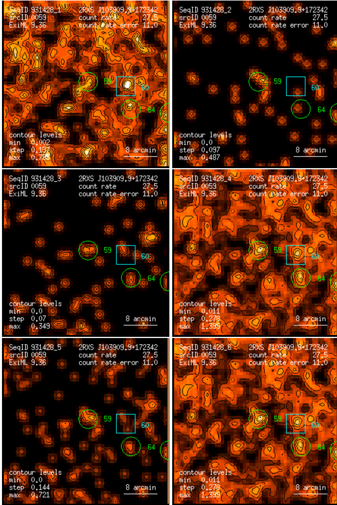
Figure 59: RASS 931428: detection 0059: band rate images, Gaussian filter: (1) PSPC channels 11 – 41, (2) 52 – 90, (3) 91 – 201, (4) 11 – 235, (5) 52 – 201, (6) 11 – 201. Broad band rates in counts/ks. Band rate contour levels in counts/ks/arcmin 2 .
