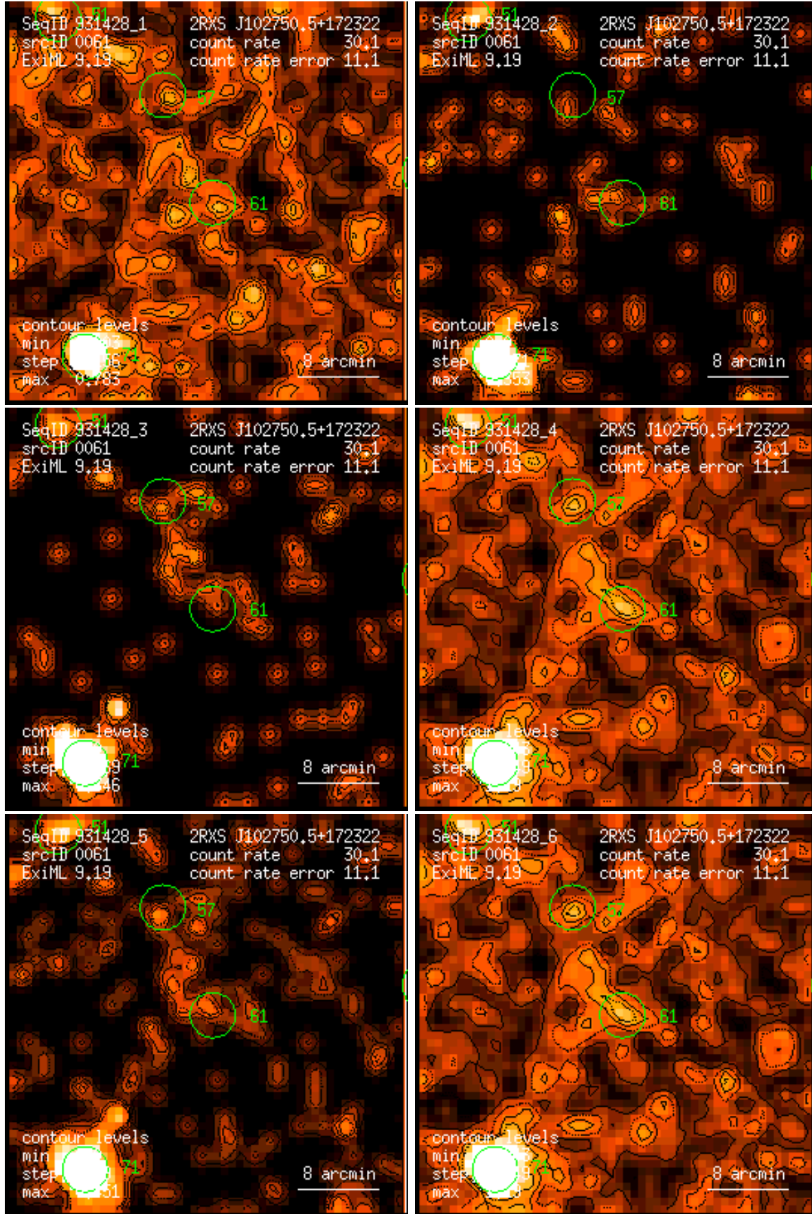
Figure 61: RASS 931428: detection 0061: band rate images, Gaussian filter: (1) PSPC channels 11 – 41, (2) 52 – 90, (3) 91 – 201, (4) 11 – 235, (5) 52 – 201, (6) 11 – 201. Broad band rates in counts/ks. Band rate contour levels in counts/ks/arcmin 2 .
