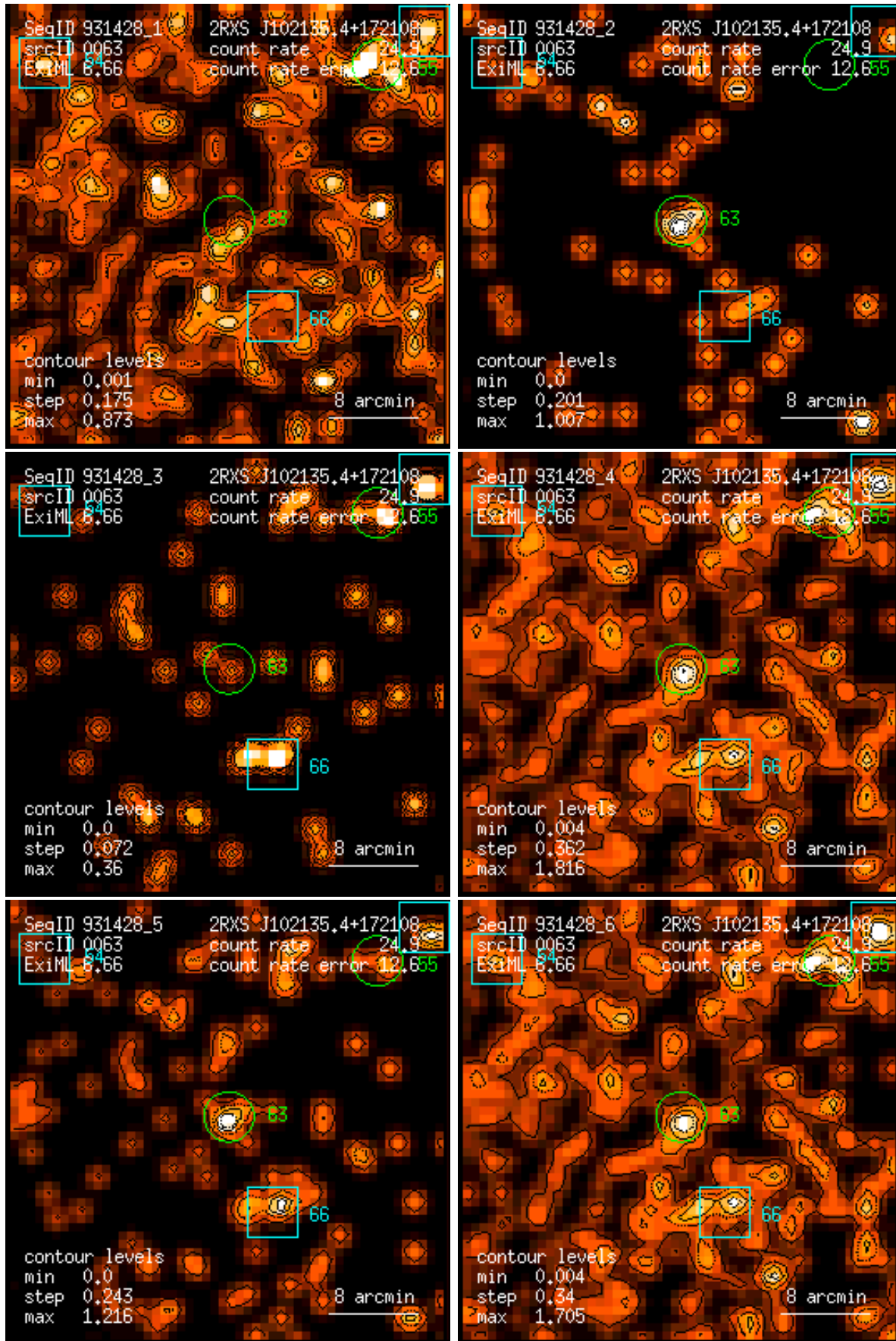
Figure 63: RASS 931428: detection 0063: band rate images, Gaussian filter: (1) PSPC channels 11 – 41, (2) 52 – 90, (3) 91 – 201, (4) 11 – 235, (5) 52 – 201, (6) 11 – 201. Broad band rates in counts/ks. Band rate contour levels in counts/ks/arcmin 2 .
