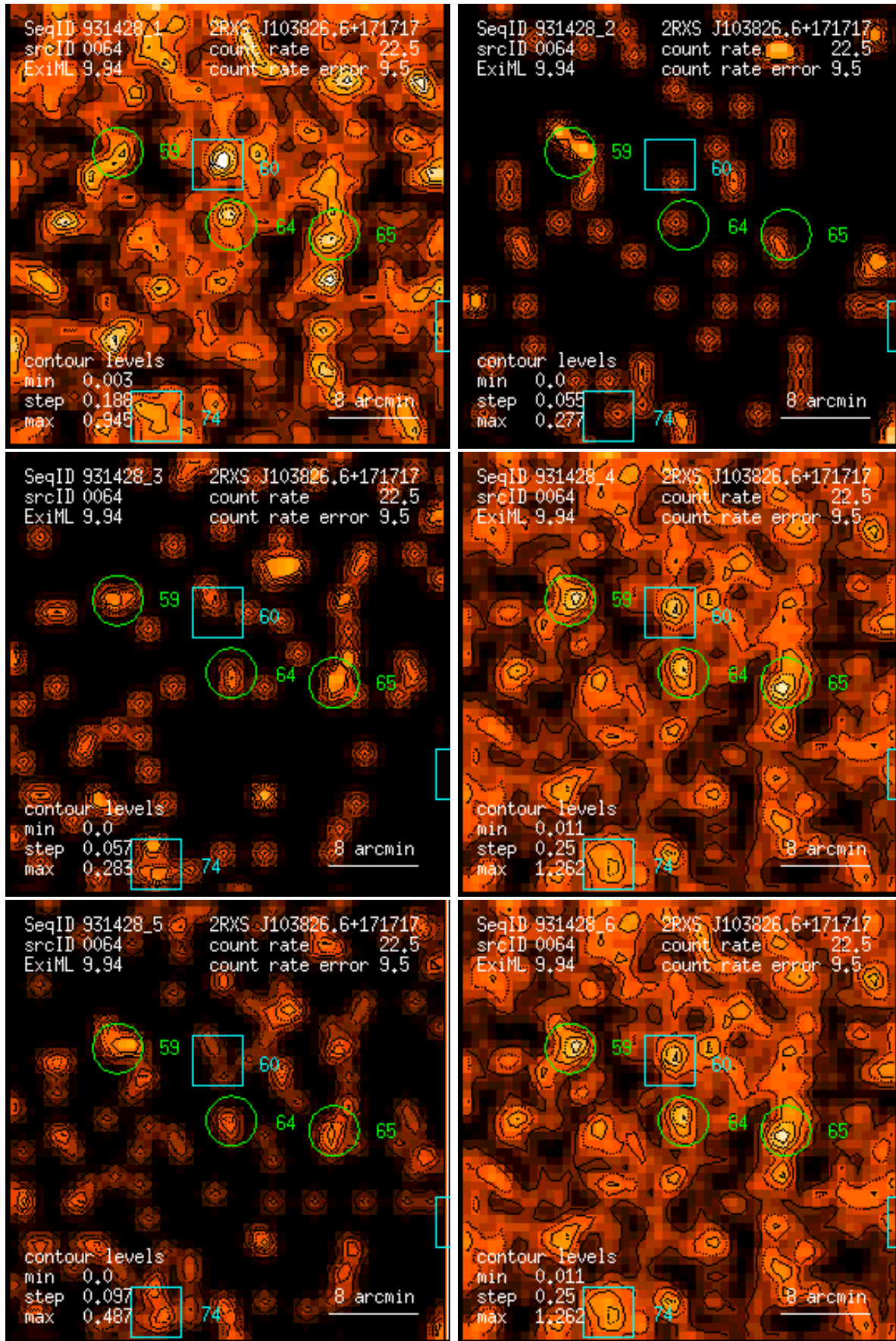
Figure 64: RASS 931428: detection 0064: band rate images, Gaussian filter: (1) PSPC channels 11 – 41, (2) 52 – 90, (3) 91 – 201, (4) 11 – 235, (5) 52 – 201, (6) 11 – 201. Broad band rates in counts/ks. Band rate contour levels in counts/ks/arcmin 2 .
