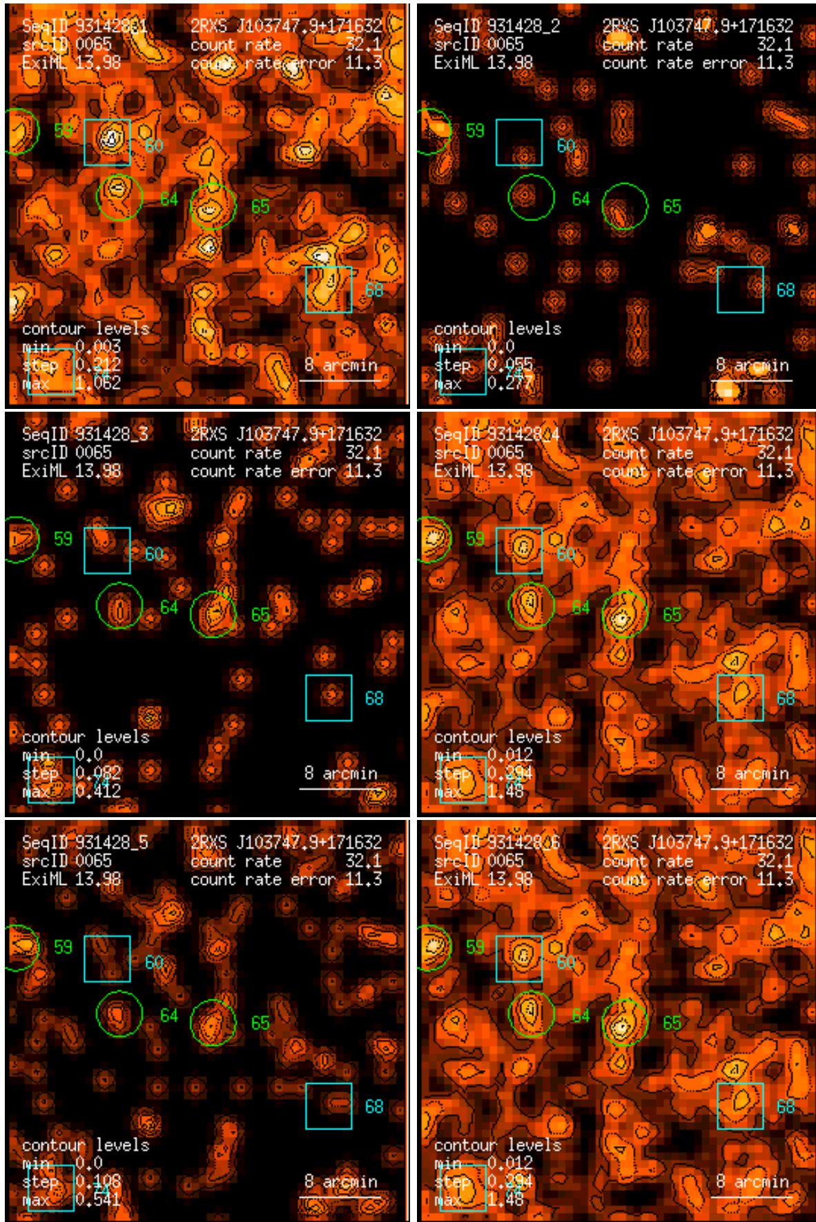
Figure 65: RASS 931428: detection 0065: band rate images, Gaussian filter: (1) PSPC channels 11 – 41, (2) 52 – 90, (3) 91 – 201, (4) 11 – 235, (5) 52 – 201, (6) 11 – 201. Broad band rates in counts/ks. Band rate contour levels in counts/ks/arcmin 2 .
