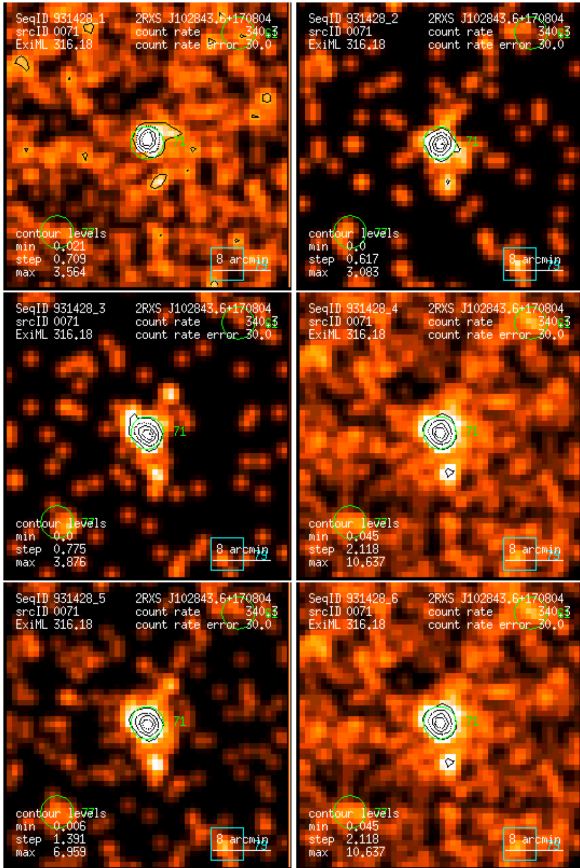
Figure 71: RASS 931428: detection 0071: band rate images, Gaussian filter: (1) PSPC channels 11 – 41, (2) 52 – 90, (3) 91 – 201, (4) 11 – 235, (5) 52 – 201, (6) 11 – 201. Broad band rates in counts/ks. Band rate contour levels in counts/ks/arcmin 2 .
