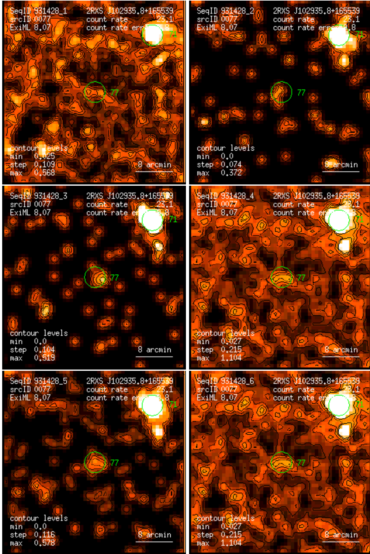
Figure 77: RASS 931428: detection 0077: band rate images, Gaussian filter: (1) PSPC channels 11 – 41, (2) 52 – 90, (3) 91 – 201, (4) 11 – 235, (5) 52 – 201, (6) 11 – 201. Broad band rates in counts/ks. Band rate contour levels in counts/ks/arcmin 2 .
