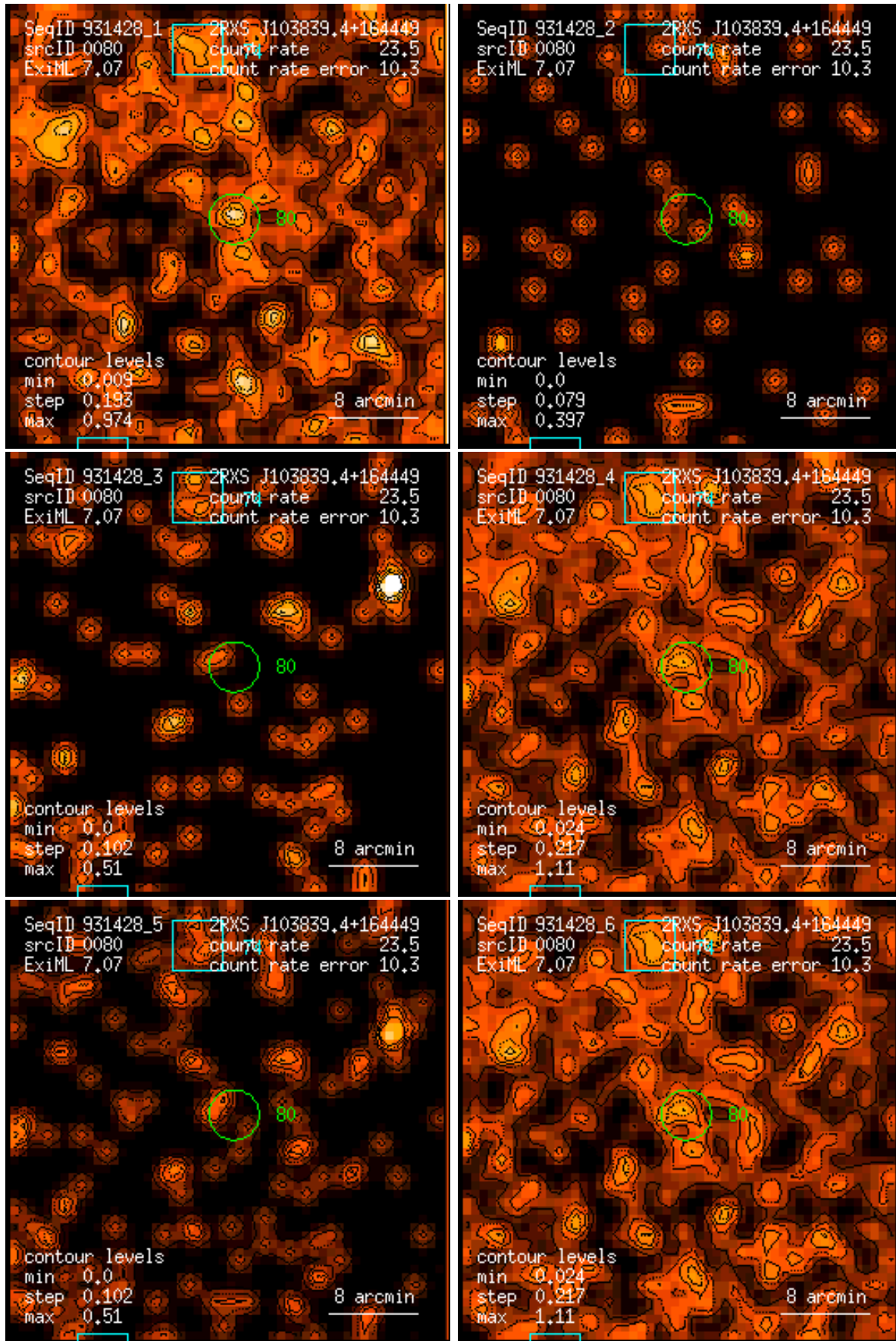
Figure 80: RASS 931428: detection 0080: band rate images, Gaussian filter: (1) PSPC channels 11 – 41, (2) 52 – 90, (3) 91 – 201, (4) 11 – 235, (5) 52 – 201, (6) 11 – 201. Broad band rates in counts/ks. Band rate contour levels in counts/ks/arcmin 2 .
