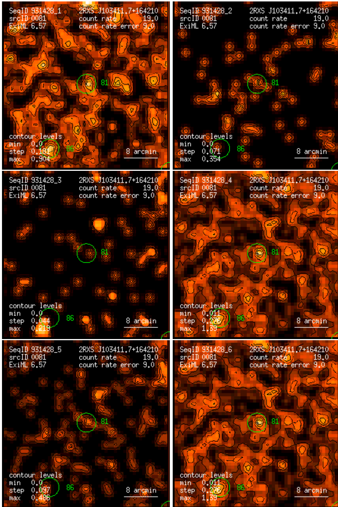
Figure 81: RASS 931428: detection 0081: band rate images, Gaussian filter: (1) PSPC channels 11 – 41, (2) 52 – 90, (3) 91 – 201, (4) 11 – 235, (5) 52 – 201, (6) 11 – 201. Broad band rates in counts/ks. Band rate contour levels in counts/ks/arcmin 2 .
