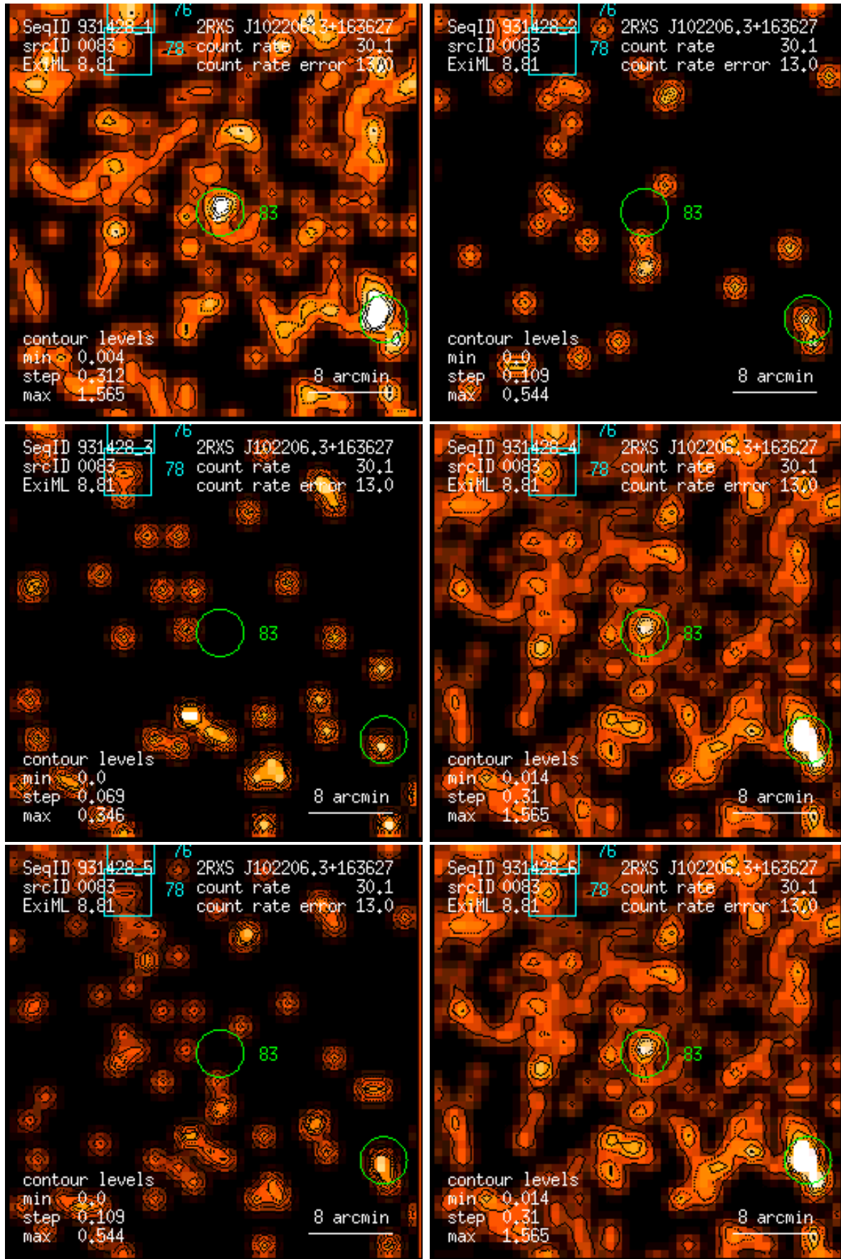
Figure 83: RASS 931428: detection 0083: band rate images, Gaussian filter: (1) PSPC channels 11 – 41, (2) 52 – 90, (3) 91 – 201, (4) 11 – 235, (5) 52 – 201, (6) 11 – 201. Broad band rates in counts/ks. Band rate contour levels in counts/ks/arcmin 2 .
