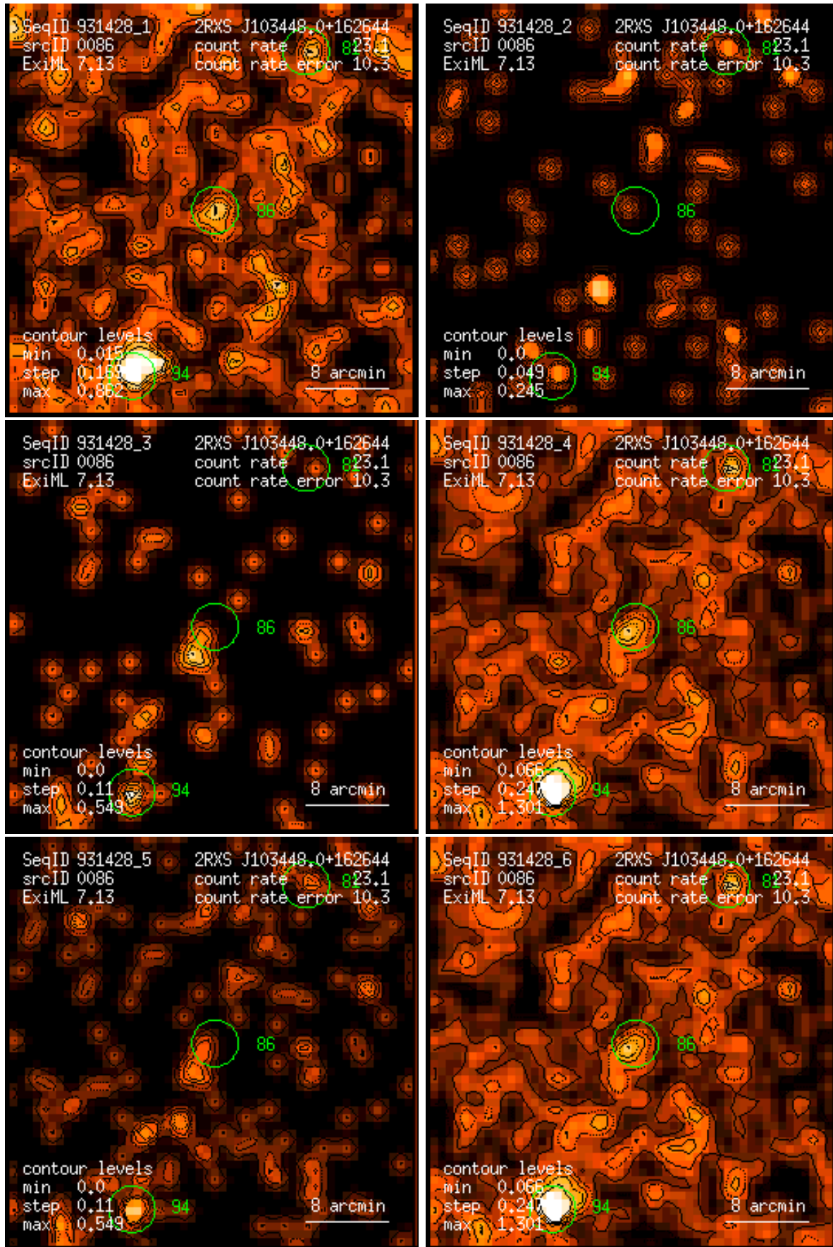
Figure 86: RASS 931428: detection 0086: band rate images, Gaussian filter: (1) PSPC channels 11 – 41, (2) 52 – 90, (3) 91 – 201, (4) 11 – 235, (5) 52 – 201, (6) 11 – 201. Broad band rates in counts/ks. Band rate contour levels in counts/ks/arcmin 2 .
