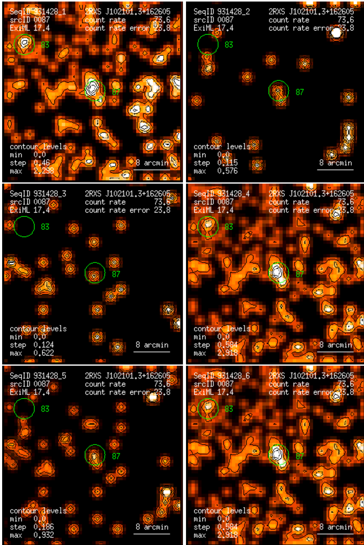
Figure 87: RASS 931428: detection 0087: band rate images, Gaussian filter: (1) PSPC channels 11 – 41, (2) 52 – 90, (3) 91 – 201, (4) 11 – 235, (5) 52 – 201, (6) 11 – 201. Broad band rates in counts/ks. Band rate contour levels in counts/ks/arcmin 2 .
