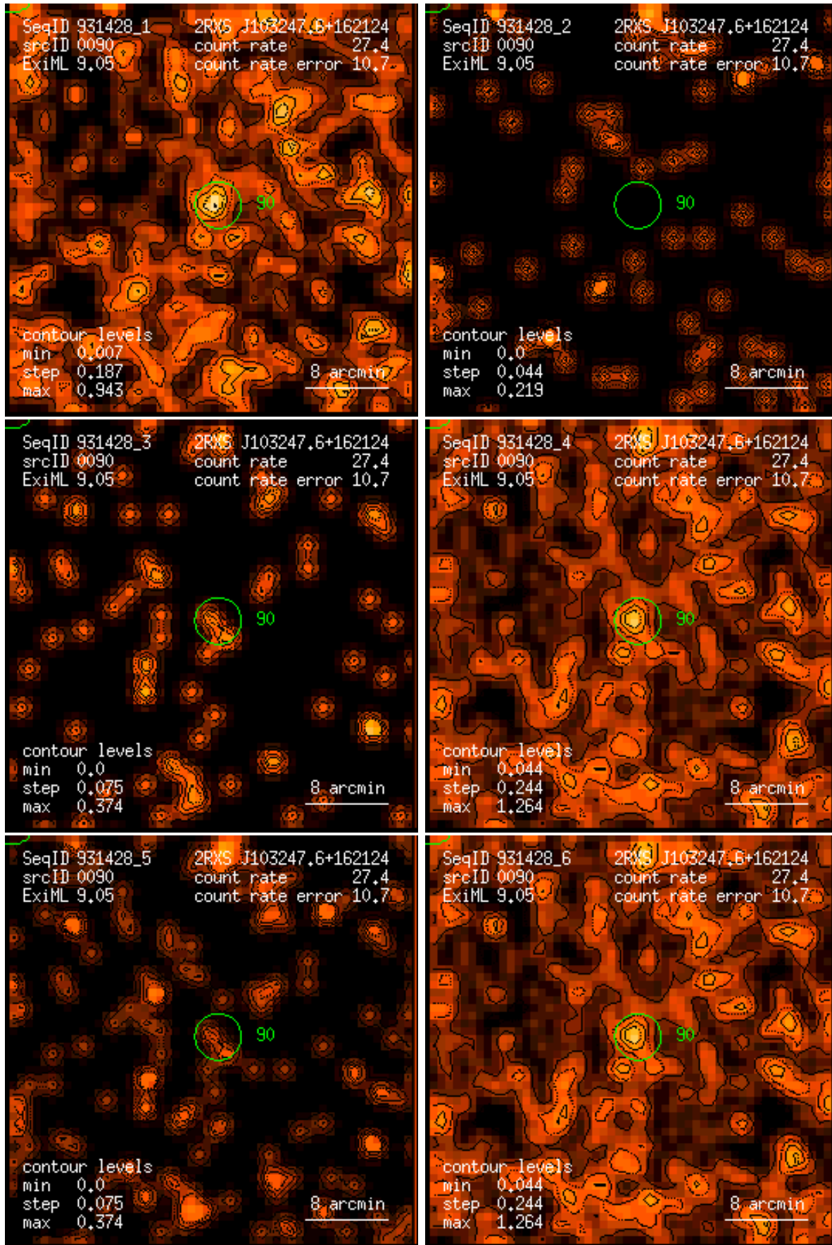
Figure 90: RASS 931428: detection 0090: band rate images, Gaussian filter: (1) PSPC channels 11 – 41, (2) 52 – 90, (3) 91 – 201, (4) 11 – 235, (5) 52 – 201, (6) 11 – 201. Broad band rates in counts/ks. Band rate contour levels in counts/ks/arcmin 2 .
