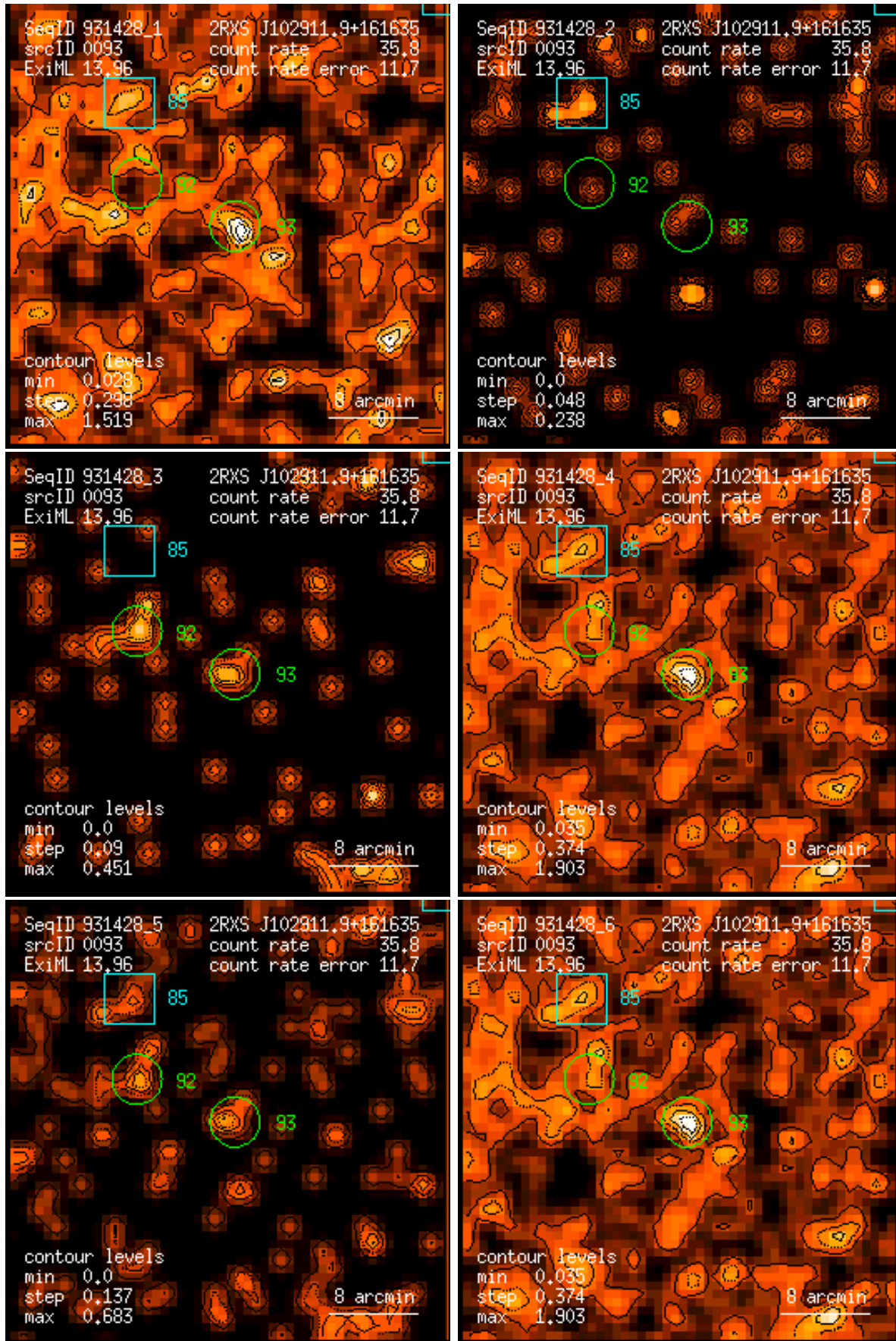
Figure 93: RASS 931428: detection 0093: band rate images, Gaussian filter: (1) PSPC channels 11 – 41, (2) 52 – 90, (3) 91 – 201, (4) 11 – 235, (5) 52 – 201, (6) 11 – 201. Broad band rates in counts/ks. Band rate contour levels in counts/ks/arcmin 2 .
