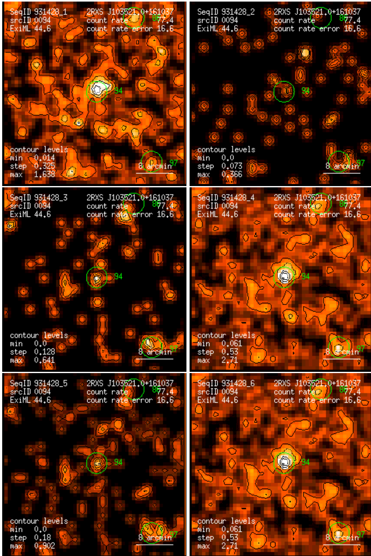
Figure 94: RASS 931428: detection 0094: band rate images, Gaussian filter: (1) PSPC channels 11 – 41, (2) 52 – 90, (3) 91 – 201, (4) 11 – 235, (5) 52 – 201, (6) 11 – 201. Broad band rates in counts/ks. Band rate contour levels in counts/ks/arcmin 2 .
