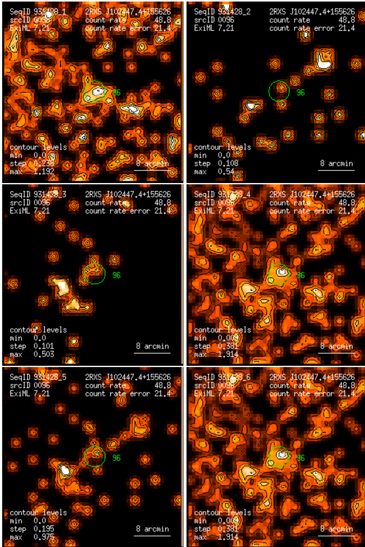
Figure 96: RASS 931428: detection 0096: band rate images, Gaussian filter: (1) PSPC channels 11 – 41, (2) 52 – 90, (3) 91 – 201, (4) 11 – 235, (5) 52 – 201, (6) 11 – 201. Broad band rates in counts/ks. Band rate contour levels in counts/ks/arcmin 2 .
