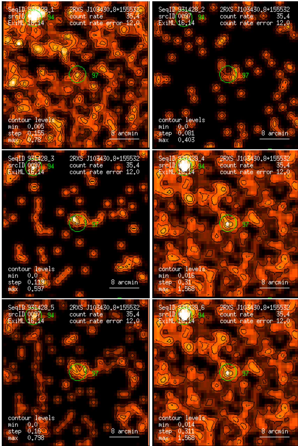
Figure 97: RASS 931428: detection 0097: band rate images, Gaussian filter: (1) PSPC channels 11 – 41, (2) 52 – 90, (3) 91 – 201, (4) 11 – 235, (5) 52 – 201, (6) 11 – 201. Broad band rates in counts/ks. Band rate contour levels in counts/ks/arcmin 2 .
