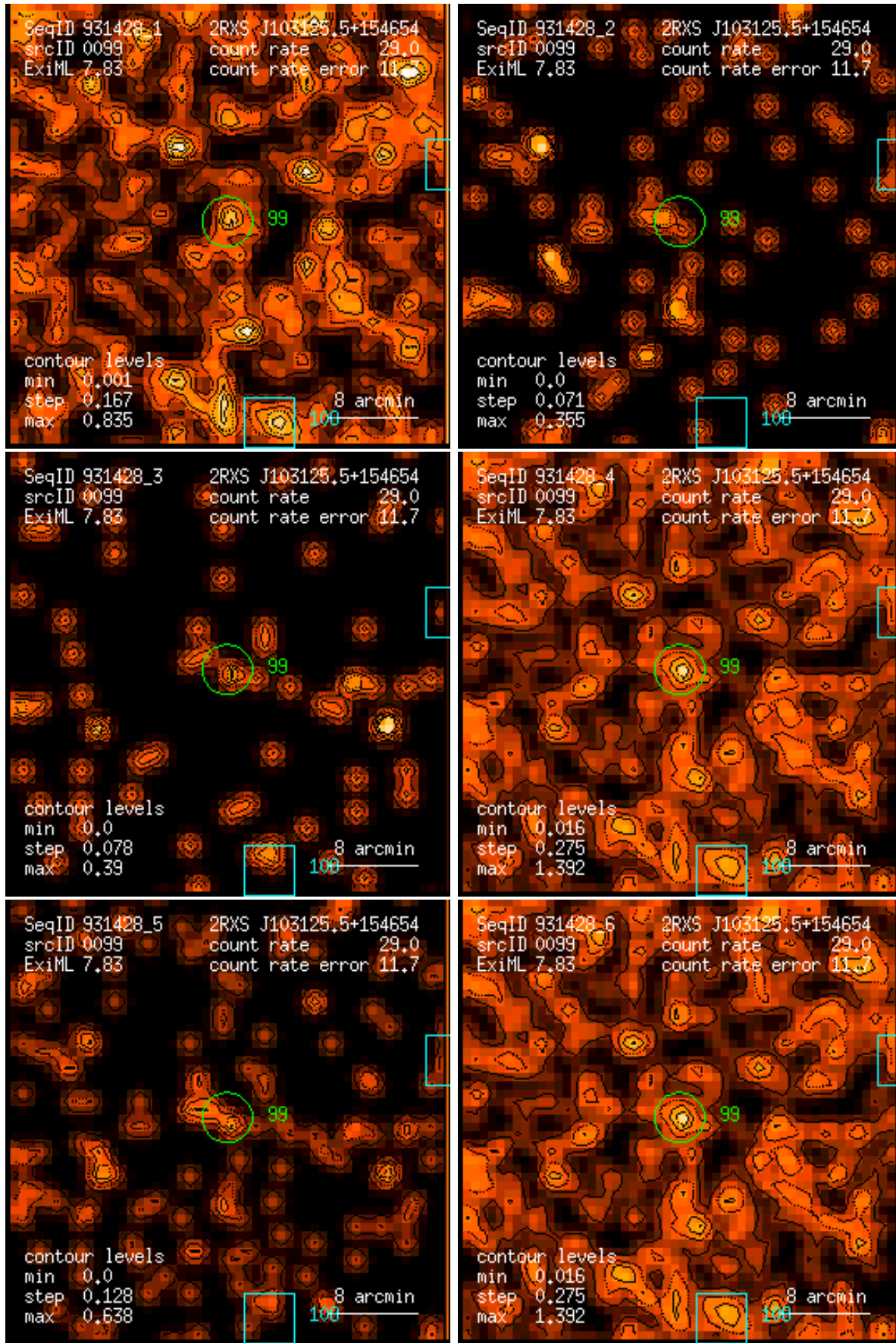
Figure 99: RASS 931428: detection 0099: band rate images, Gaussian filter: (1) PSPC channels 11 – 41, (2) 52 – 90, (3) 91 – 201, (4) 11 – 235, (5) 52 – 201, (6) 11 – 201. Broad band rates in counts/ks. Band rate contour levels in counts/ks/arcmin 2 .
