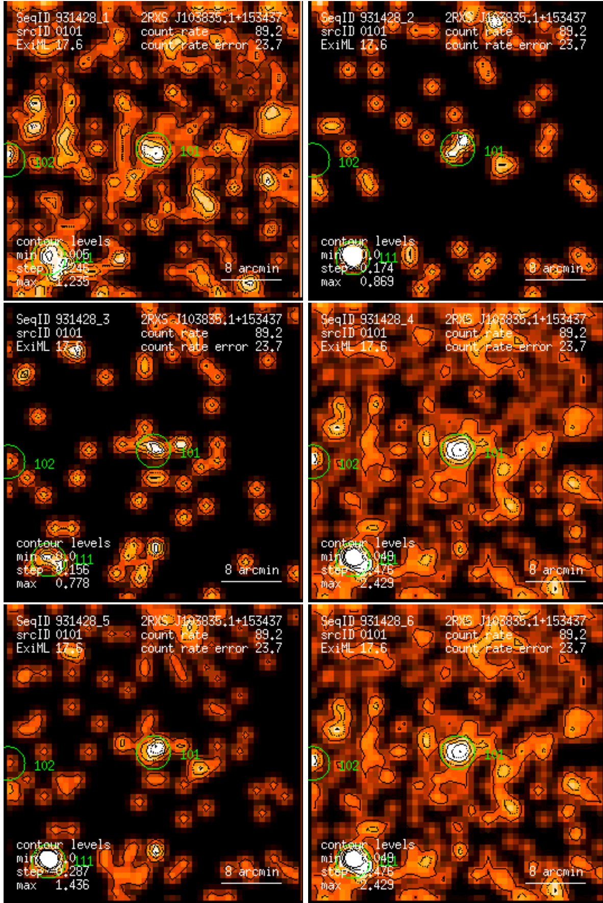
Figure 101: RASS 931428: detection 0101: band rate images, Gaussian filter: (1) PSPC channels 11 – 41, (2) 52 – 90, (3) 91 – 201, (4) 11 – 235, (5) 52 – 201, (6) 11 – 201. Broad band rates in counts/ks. Band rate contour levels in counts/ks/arcmin 2 .
