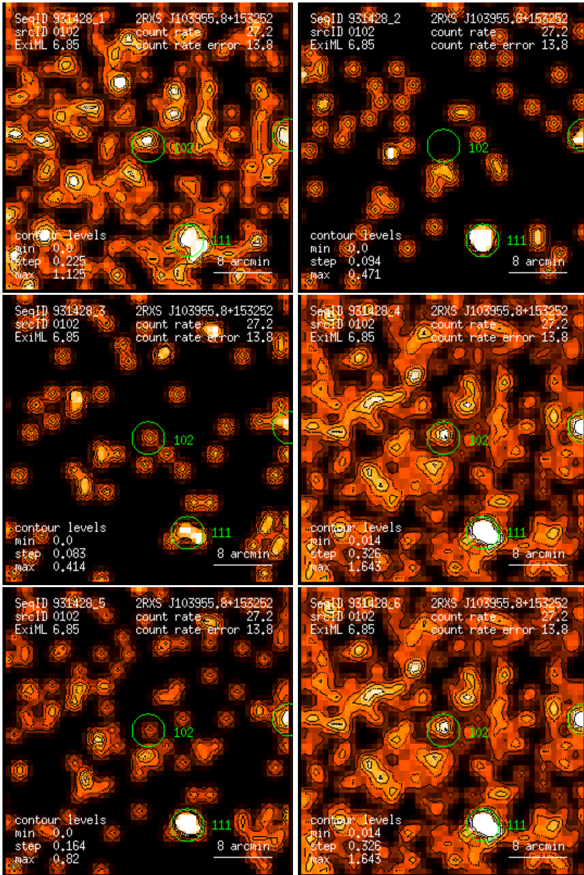
Figure 102: RASS 931428: detection 0102: band rate images, Gaussian filter: (1) PSPC channels 11 – 41, (2) 52 – 90, (3) 91 – 201, (4) 11 – 235, (5) 52 – 201, (6) 11 – 201. Broad band rates in counts/ks. Band rate contour levels in counts/ks/arcmin 2 .
