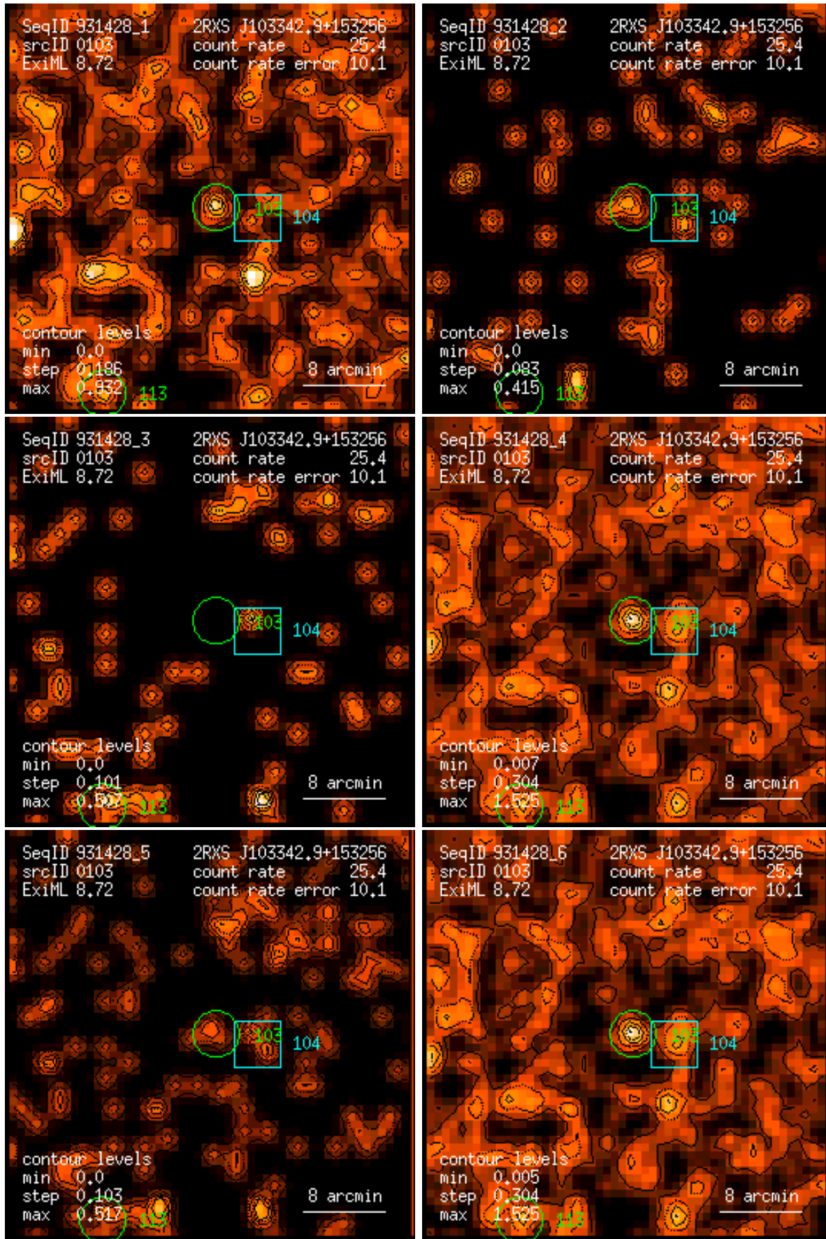
Figure 103: RASS 931428: detection 0103: band rate images, Gaussian filter: (1) PSPC channels 11 – 41, (2) 52 – 90, (3) 91 – 201, (4) 11 – 235, (5) 52 – 201, (6) 11 – 201. Broad band rates in counts/ks. Band rate contour levels in counts/ks/arcmin 2 .
