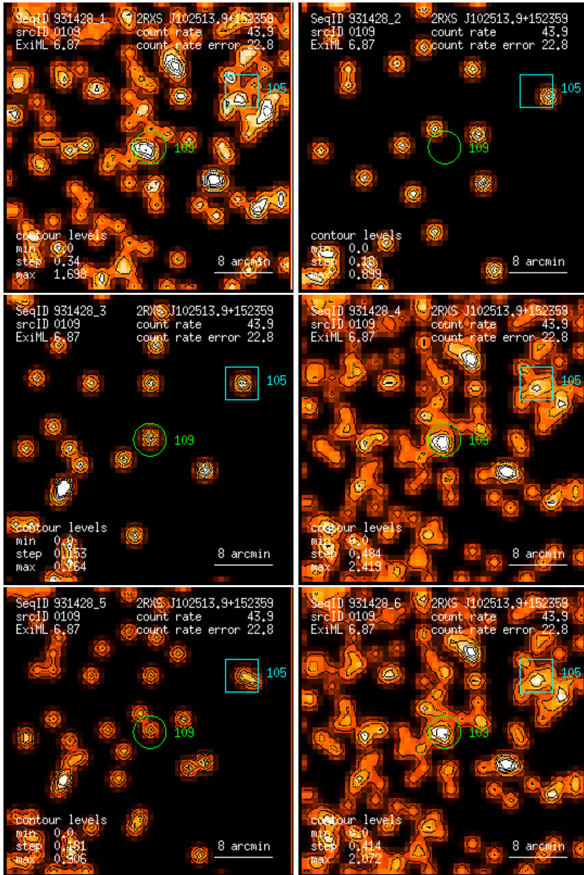
Figure 109: RASS 931428: detection 0109: band rate images, Gaussian filter: (1) PSPC channels 11 – 41, (2) 52 – 90, (3) 91 – 201, (4) 11 – 235, (5) 52 – 201, (6) 11 – 201. Broad band rates in counts/ks. Band rate contour levels in counts/ks/arcmin 2 .
