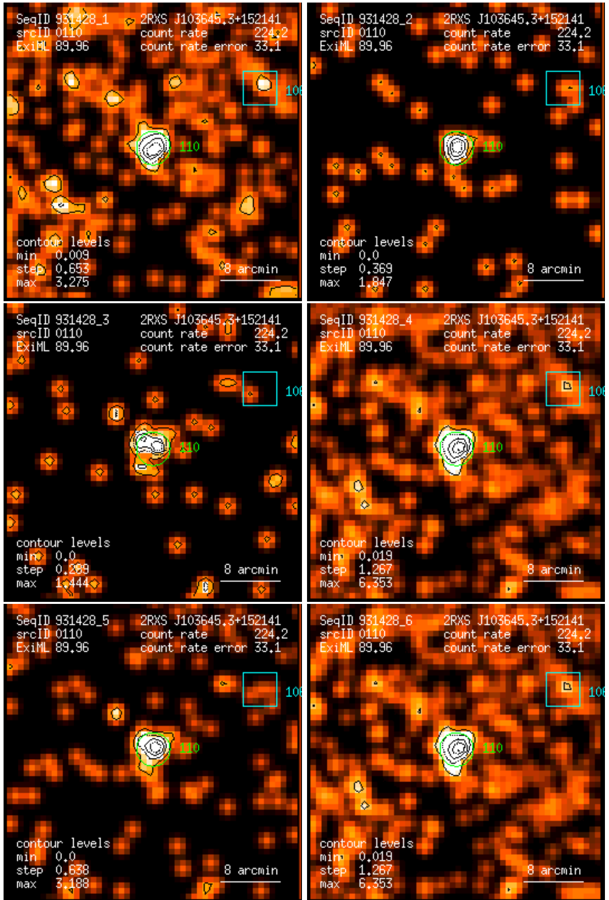
Figure 110: RASS 931428: detection 0110: band rate images, Gaussian filter: (1) PSPC channels 11 – 41, (2) 52 – 90, (3) 91 – 201, (4) 11 – 235, (5) 52 – 201, (6) 11 – 201. Broad band rates in counts/ks. Band rate contour levels in counts/ks/arcmin 2 .
