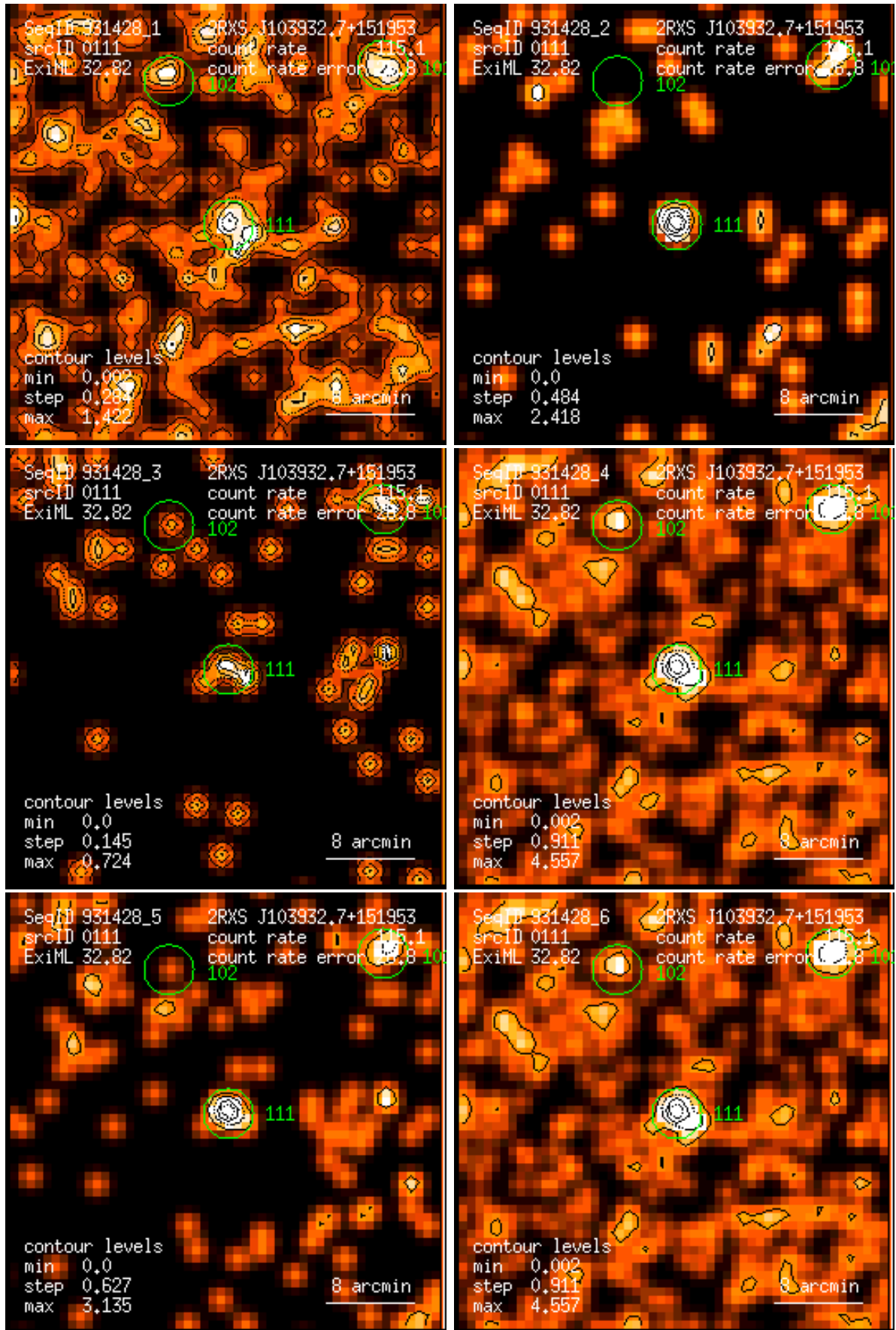
Figure 111: RASS 931428: detection 0111: band rate images, Gaussian filter: (1) PSPC channels 11 – 41, (2) 52 – 90, (3) 91 – 201, (4) 11 – 235, (5) 52 – 201, (6) 11 – 201. Broad band rates in counts/ks. Band rate contour levels in counts/ks/arcmin 2 .
