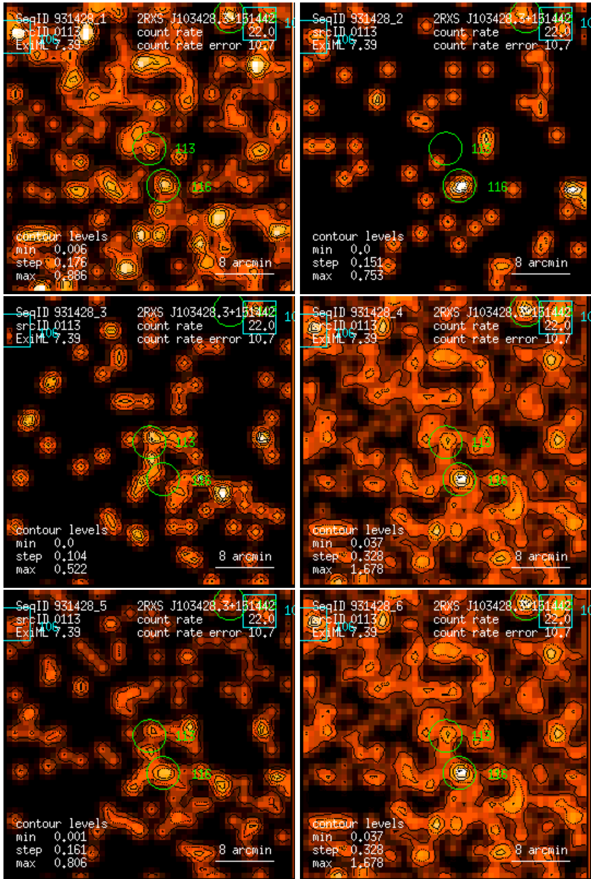
Figure 113: RASS 931428: detection 0113: band rate images, Gaussian filter: (1) PSPC channels 11 – 41, (2) 52 – 90, (3) 91 – 201, (4) 11 – 235, (5) 52 – 201, (6) 11 – 201. Broad band rates in counts/ks. Band rate contour levels in counts/ks/arcmin 2 .
