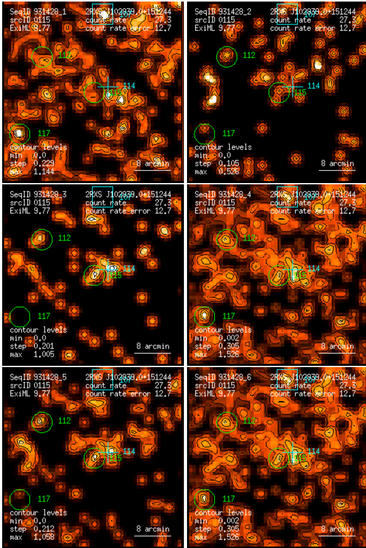
Figure 115: RASS 931428: detection 0115: band rate images, Gaussian filter: (1) PSPC channels 11 – 41, (2) 52 – 90, (3) 91 – 201, (4) 11 – 235, (5) 52 – 201, (6) 11 – 201. Broad band rates in counts/ks. Band rate contour levels in counts/ks/arcmin 2 .
