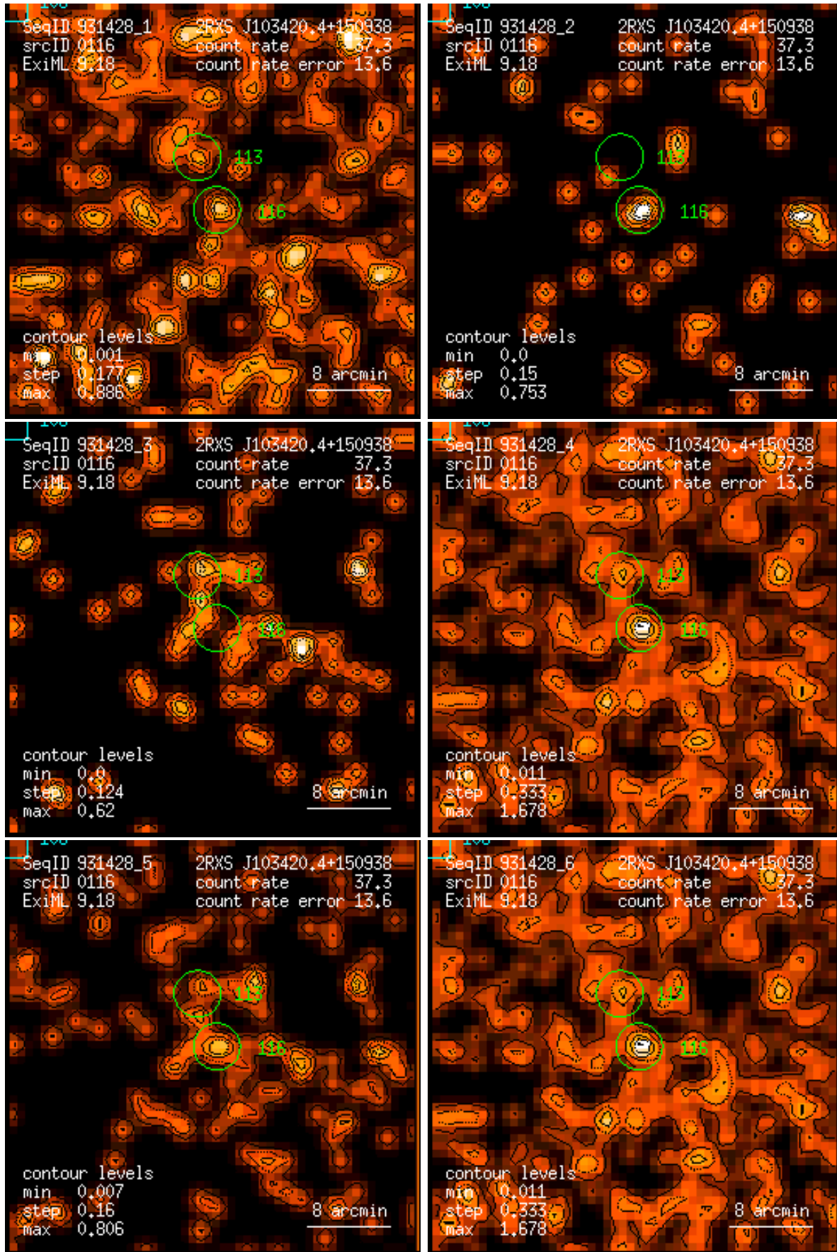
Figure 116: RASS 931428: detection 0116: band rate images, Gaussian filter: (1) PSPC channels 11 – 41, (2) 52 – 90, (3) 91 – 201, (4) 11 – 235, (5) 52 – 201, (6) 11 – 201. Broad band rates in counts/ks. Band rate contour levels in counts/ks/arcmin 2 .
