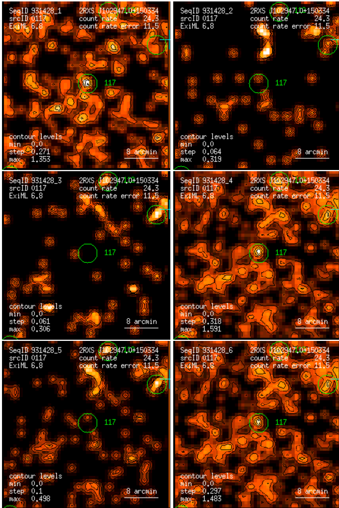
Figure 117: RASS 931428: detection 0117: band rate images, Gaussian filter: (1) PSPC channels 11 – 41, (2) 52 – 90, (3) 91 – 201, (4) 11 – 235, (5) 52 – 201, (6) 11 – 201. Broad band rates in counts/ks. Band rate contour levels in counts/ks/arcmin 2 .
