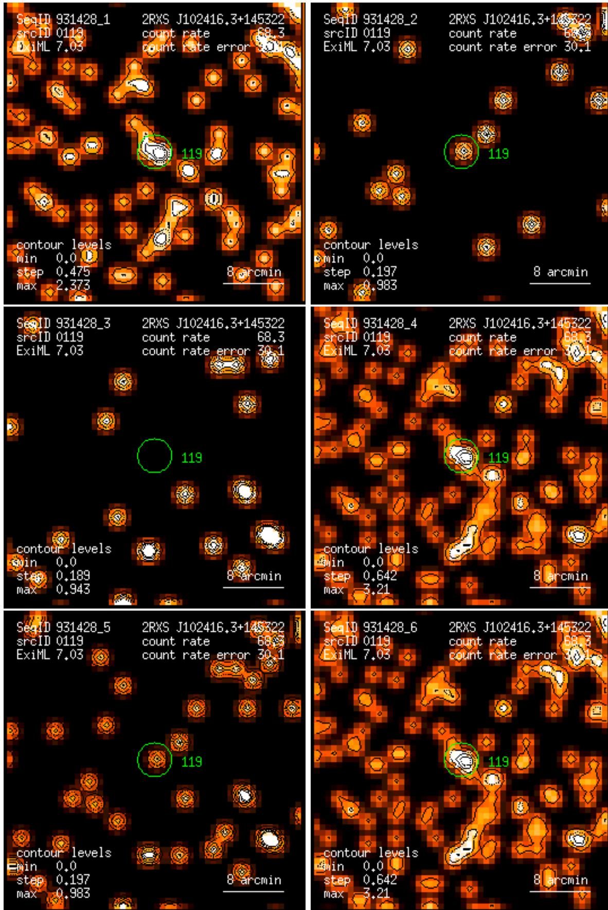
Figure 119: RASS 931428: detection 0119: band rate images, Gaussian filter: (1) PSPC channels 11 – 41, (2) 52 – 90, (3) 91 – 201, (4) 11 – 235, (5) 52 – 201, (6) 11 – 201. Broad band rates in counts/ks. Band rate contour levels in counts/ks/arcmin 2 .
